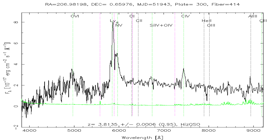
Figure 4.9: Absorption spectrum of a quasar observed by the SDSS telescope, published on the third release. The quasar is at z=3.81 . Also plotted, the continuum spectra and the relevant absorption lines [89].
