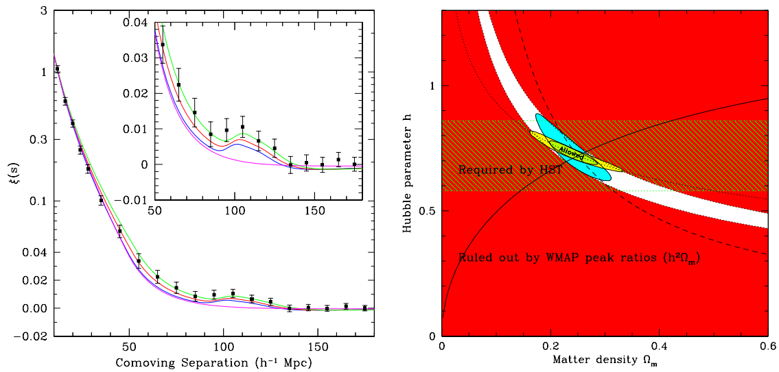
Figure 4.4: ( Left ) This figure has been directly extracted from [87] and shows the experimental points in the correlation function of the SDSS-LRG sample. It is plotted along three theoretical predictions corresponding to \Omega_M h^2 = 0.12 (top, green), 0.13 (red), and 0.14 (bottom with peak, blue), all with \omega_B = 0.024 and n = 0.98 . The magenta line shows a pure CDM model ( \Omega_M h^2 = 0.105 ), which lacks the acoustic peak (see [87] for a detailed explanation). ( Right ) This figure has been directly extracted from [90] and illustrates how the BAO measurement helps breaking the degeneracy in the \Omega_M - h plane present in any CMB-only analysis (See [90] and text for details).
