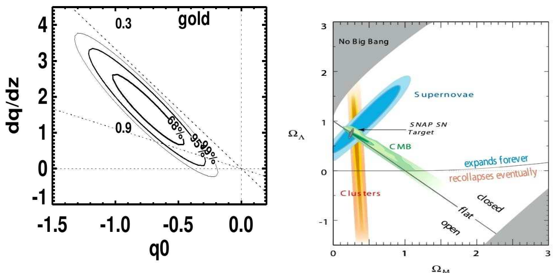
Figure 4.7: Predicted contour likelihood for the SNAP experiment (grey) compared to the rest of the constrains in the \Omega_M - \Omega_\Lambda parameter space [100].
