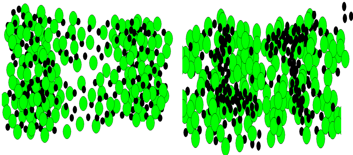
Figure 3.1: Artistic photon and neutrino soup. On the left hand side, the background energy density spatially fluctuates. However, the ratio n_\gamma/n_\nu has a constant value in space. On the right hand side, we encounter the opposite scenario. Even though the background energy density is constant, n_\gamma/n_\nu fluctuates throughout space.
