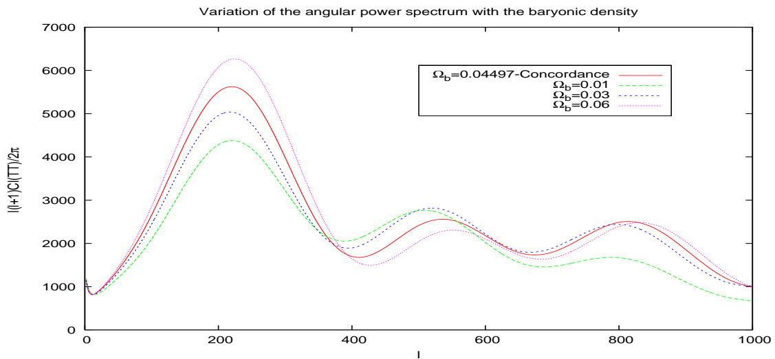
Figure 4.3: Variation of the height of the 1 st and the 3 rd peaks with \Omega_b .
