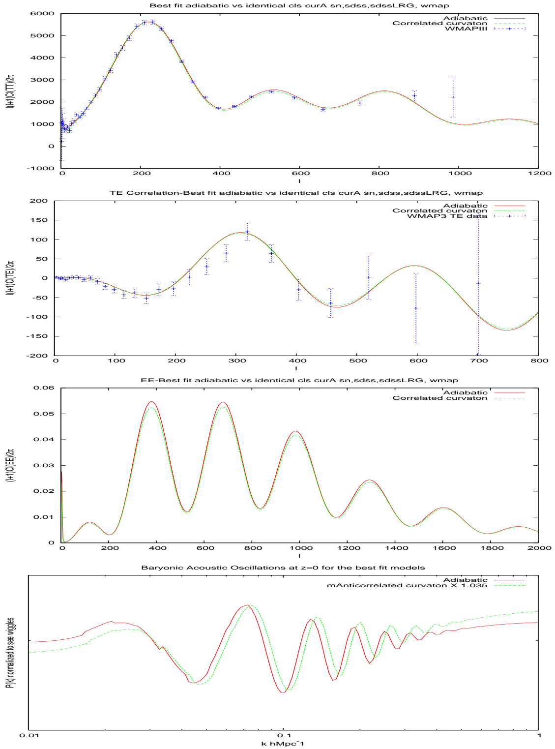
Figure 4.5: Different power spectra for the models described on Table 4.1. In the bottom panel, the amplitude of the isocurvature spectrum has been increased by 3.5% to show more clearly the shifts on the peaks.
