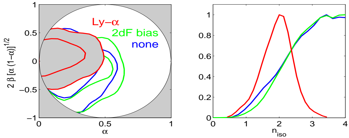
Figure 6.7: Likelihood of the isocurvature-related parameters, for the three combinations of data sets described in section 6.2.1: “Lyman- \alpha ” (red), “2dF bias prior” (green) and “none” (blue). (Left) Marginalized 1\sigma and 2\sigma confidence levels in the (\alpha, 2\beta[\alpha(1-\alpha)]^{1/2}) space. (Right) Marginalized probability distribution for n_{\text{iso}} .
