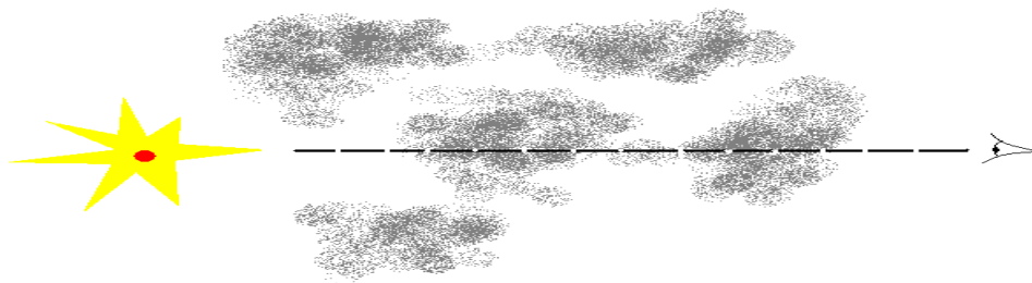
Figure 4.8: Illustration to show how the spectrum of the quasar determines the position and densities of the absorbers encountered in the way.
