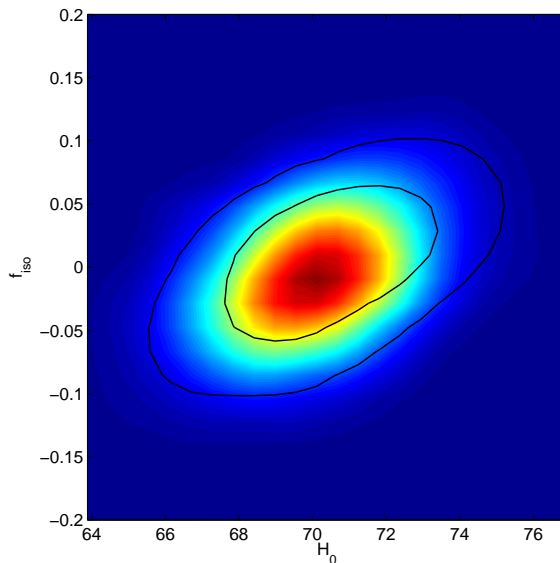
Figure 4.6: Degeneracy on the H - f_{\text{iso}} plane for both the correlated and anti-correlated case.
