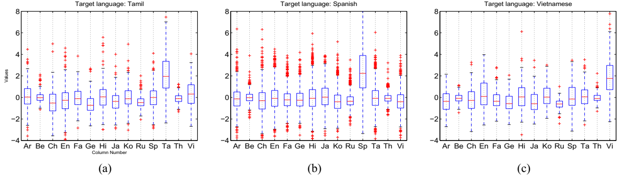
Figure 2: Distributions of scores in the form of box plots over 14 detection tasks against pretrained models m_j , j \in \{\text{arabic, bengali, chinese, english, farsi, german, hindustani, japanese, korean, russian, spanish, tamil, thai, vietnamese}\} for Tamil (a), Spanish (b) and Vietnamese (c) utterances.
