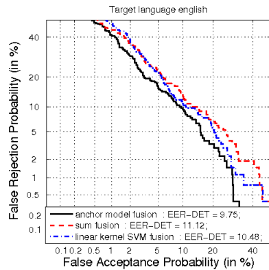
Figure 5: Results for the three fusion schemes tested: linear kernel SVM, sum fusion and AMF. DETs are shown for english model ( m'_{english} ) and 30 sec. test segments.
