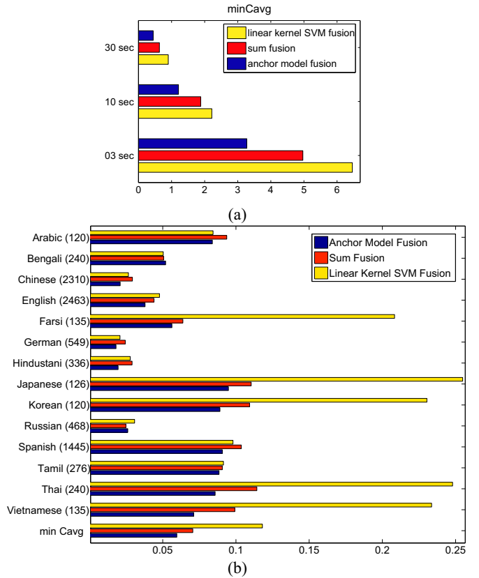
Figure 4: C_{avg} for anchor model, sum and linear kernel SVM fusions. Results are divided by test segment durations (a), and detailed per language for 30 sec. test utterances (b). Brackets show the number of utterances used to train each model.
