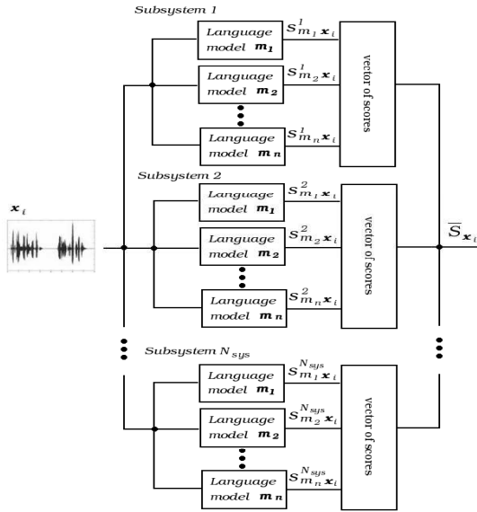
Figure 3: Schematic diagram of generation of features (scores) in the anchor model space. \bar{S}_{x,m} stacks the similarities of x_i over the set of models m_j^l , for language j and subsystem l
