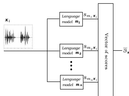
Figure 1: Schematic of n -class parallel language detection problem. \bar{S}_{x_i} stacks the similarities of x_i over the set of m_j .
