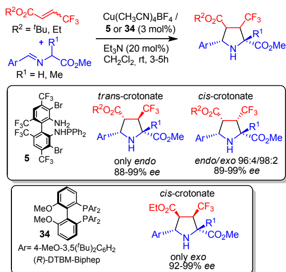
Scheme 15. Cu(I)/(S)-TF-BiphamPhos catalyzed cycloaddition with trifluorocrotonates
