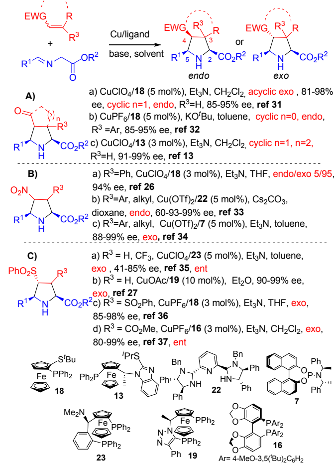
Scheme 9. Copper-catalyzed 1,3-dipolar cycloaddition of azomethine ylides with enones, nitroalkenes and vinylsulfones.
