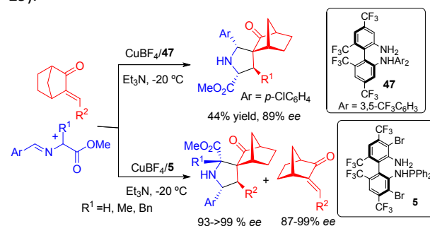
Scheme 27. Metal controlled enantiodivergent 1,3-dipolar cycloaddition of azomethine ylides with acrylates
