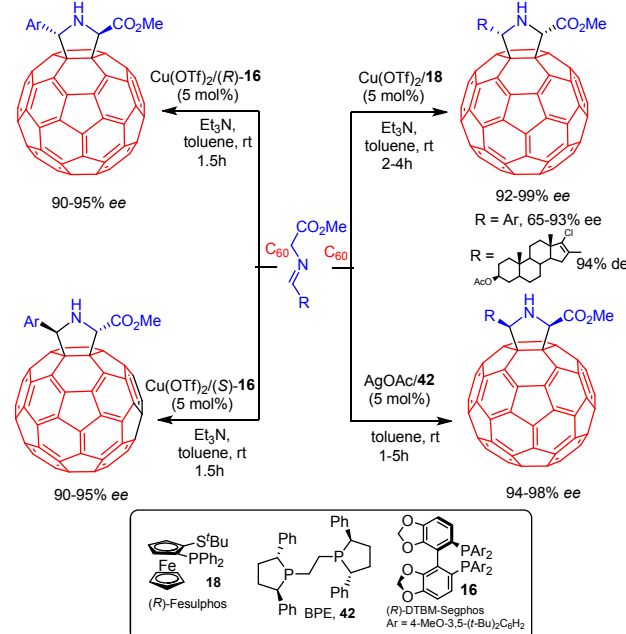
Scheme 22. Fullerenes as dipolarophiles
