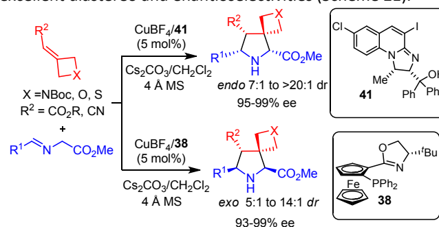
Scheme 21. Diastereodivergent synthesis of spirocyclic pyrrolidines.
