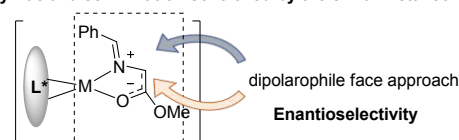
Scheme 1. Controlling factors on the stereochemical outcome of metal-catalyzed asymmetric 1,3-dipolar cycloaddition of stabilized azomethine ylides
