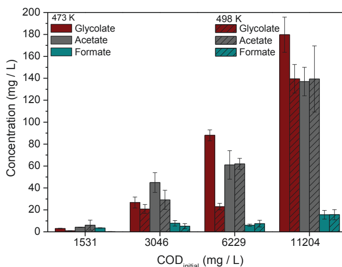
Figure 5. Main anions detected at 473 and 498 K at different organic load a
