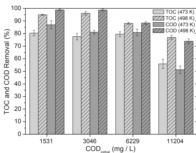
Figure 4. TOC and COD removal upon APR at 473 and 498 K at different organic load a
