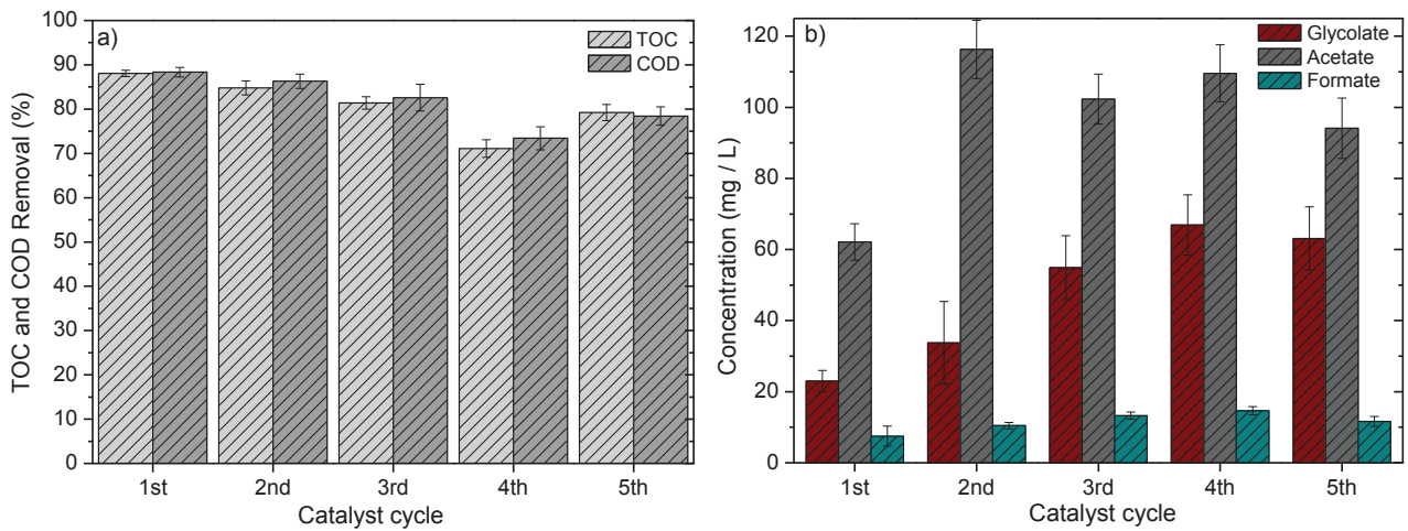
Figure 6. a) TOC and COD removal and b) anions detected upon 5 successive APR cycles a
