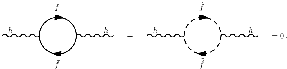
Figure 1.1.1: Left: A Higgs boson dissociating into a virtual fermion-antifermion pair in the Standard Model. Right: A Higgs boson dissociating into a virtual sfermion-antisfermion pair. This diagram cancels the one on the left.
