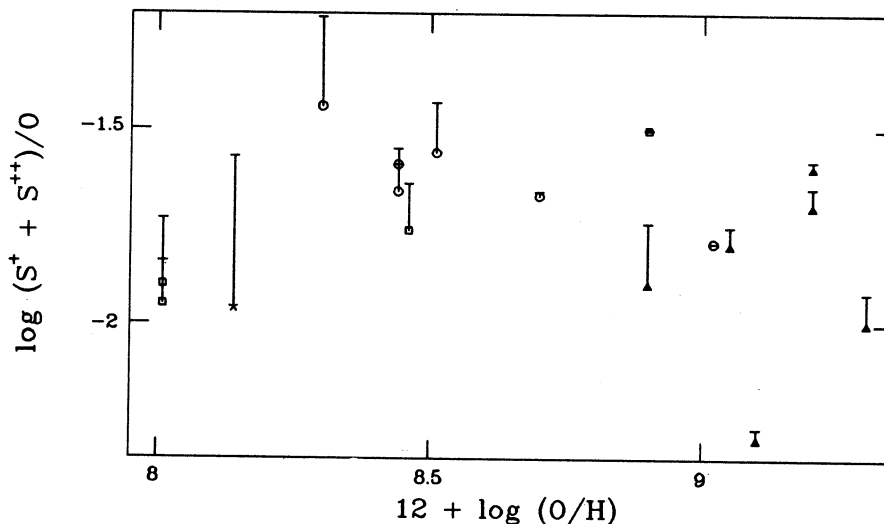
Fig.3. \log(S^+ + S^{++})/O versus 12 + \log O/H ; o: M33, \Delta : M51, \square : M101, *: IIZw 40.
