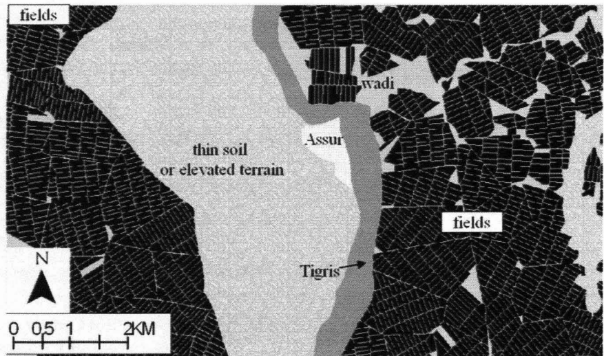
Fig. 5. Computer generated image showing some of the simulated Assur area. This image was derived using the spatial data discussed. Agricultural fields are shown as dark colored shapes, with thin soil and elevated terrains shown as gray and light gray features.
