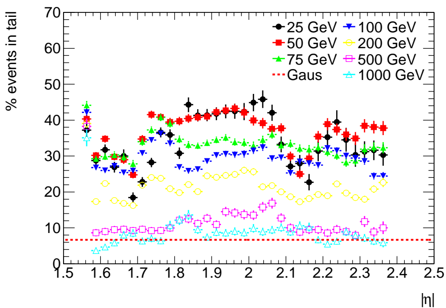
Figure 7.19: Fraction of events in the low energy tails as vs \eta for converted photons of various energies.
