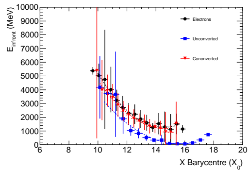
(b) 50 GeV particles
