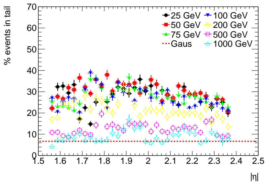
Figure 7.17: Fraction of events in the low energy tails as vs \eta for electrons of various energies.
