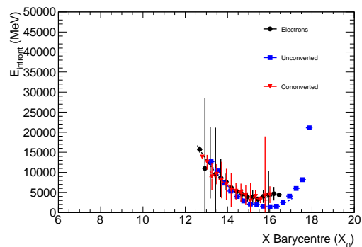
(f) 500 GeV particles
