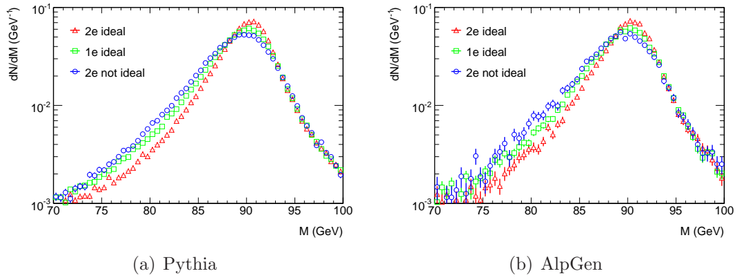
Figure 8.9: Zoom to the peak of the mass distribution for the different sub-samples and the combination.
