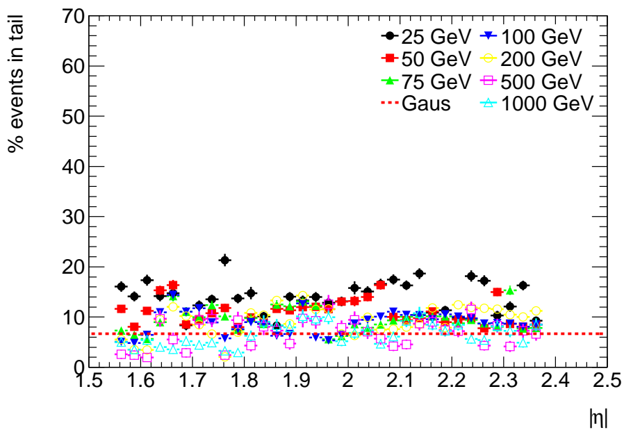
Figure 7.18: Fraction of events in the low energy tails as vs \eta for unconverted photons of various energies.
