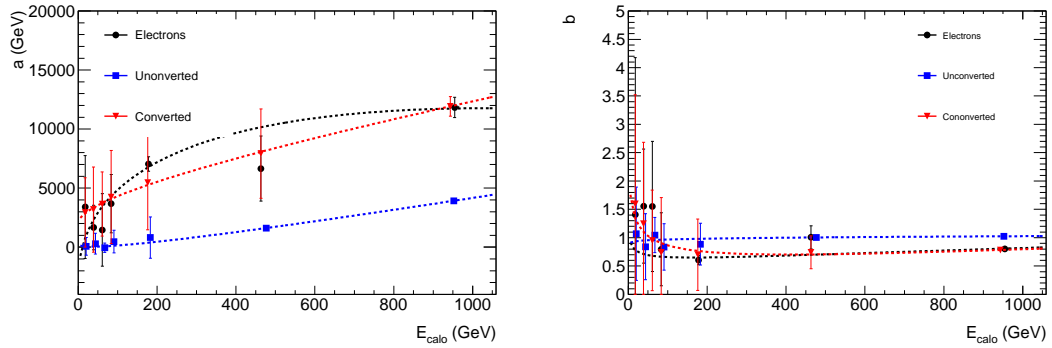
(a) a versus E_{calo}
