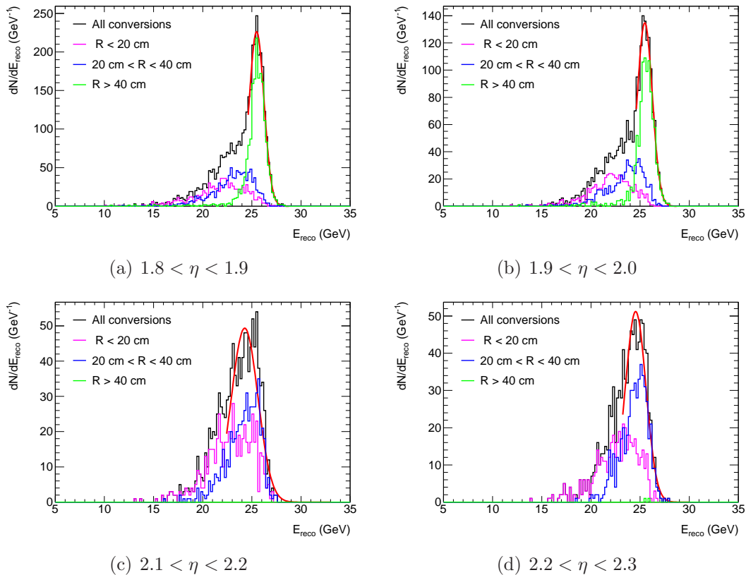
Figure 7.25: Energy distributions for converted photons
