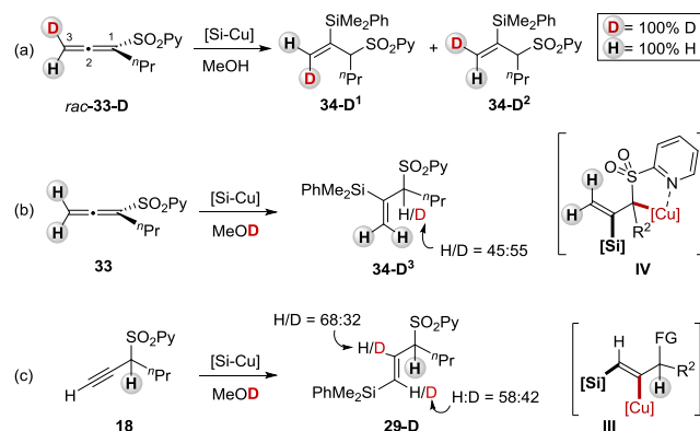
Scheme 4. D-labeling studies on the reaction mechanism.
