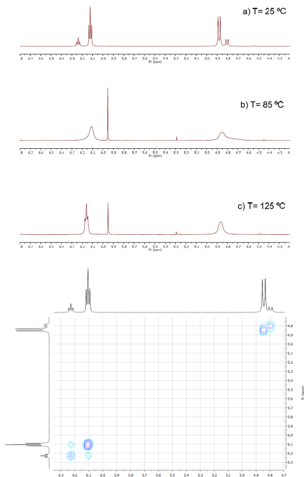
Figure 1. Olefinic and allylic peaks attributed to rotamers in compound 42 . (i) Coalescence of at higher temperature. (ii) Exchange cross-peaks observed in a 2D NOESY experiment.
