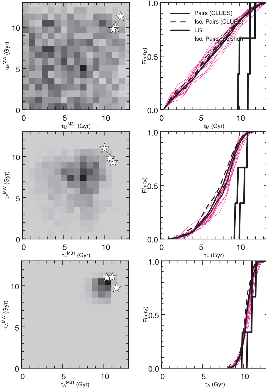
Figure 4. Left column: joint distributions of three different times (last major merger, formation and assembly) describing the MAHs. Each point in the plane represents a pair MW–M31 with histories described by the time values at that point. Levels in shading coding indicate the number of halo pairs in the Bolshoi simulations in that parameter range. Dark regions represent a high number of pairs. An absolute scaling for this shading can be obtained from the plots presented in the right column. The stars mark the location of the three LG pairs, each one coming from one of the constrained simulations. Right column: integrated probability of these three different MAH times. The continuous black lines represent the results for the Pairs sample in the CLUES simulations. The Isolated Pairs sample from CLUES is represented by the thick dashed lines. The results from the Isolated Pairs samples in eight subvolumes of the Bolshoi simulation are represented by the thin continuous grey lines. The thick continuous lines represent the results for the LG sample. The distributions from the Pairs and Isolated Pairs control samples are basically indistinguishable. In other words, detailed selection criteria for halo pairs, based on isolation only, do not narrow down significantly the range of dark matter halo assembly properties.
