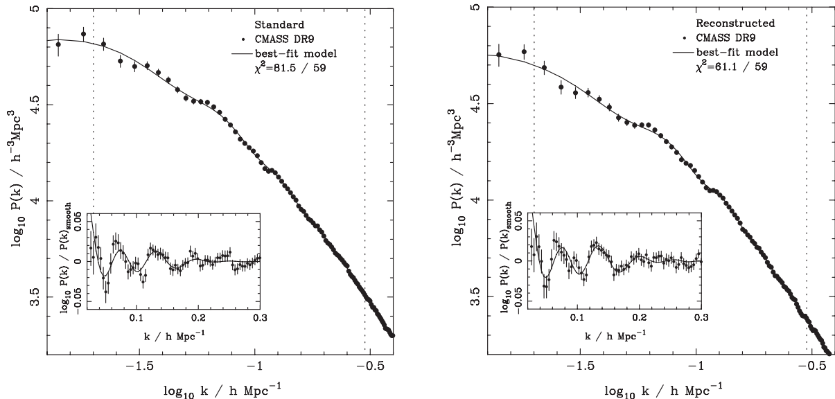
Figure 8. The CMASS DR9 power spectra before (left) and after (right) reconstruction with the best-fitting models overplotted. The vertical dotted lines show the range of scales fitted ( 0.02 < k < 0.3 h \text{Mpc}^{-1} ), and the inset shows the BAO within this k -range, determined by dividing both model and data by the best-fitting model calculated (including window function convolution) with no BAO. Error bars indicate \sqrt{C_{ii}} for the power spectrum and the rms error calculated from fitting BAO to the 600 mocks in the inset (see Section 4.2 for details).
