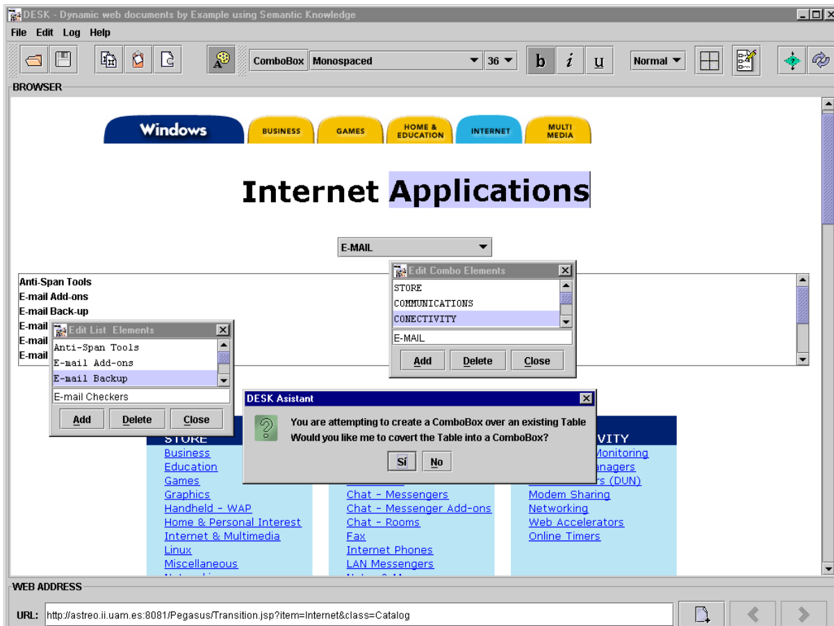
Figure 6. DESK authoring tool in editing mode
