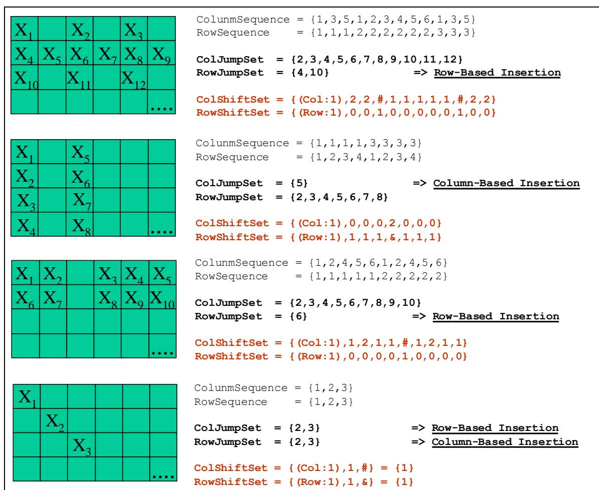
Figure 10. Some examples of iteration patterns detected by IP Algorithms
