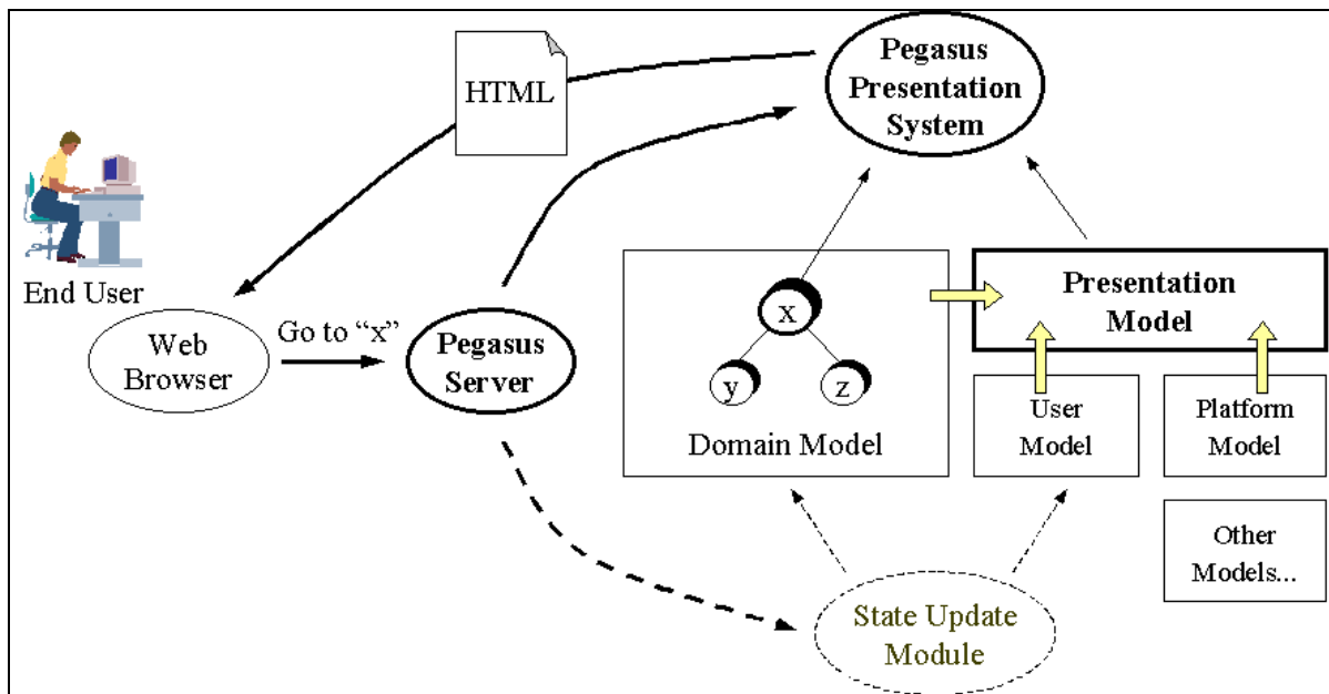
Figure 2. PEGASUS Architecture
