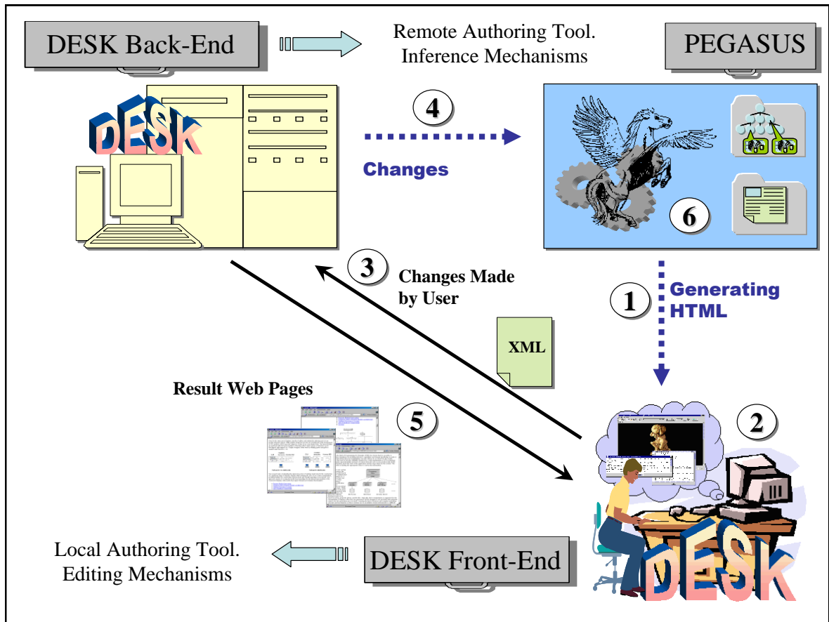
Figure 3. DESK mechanism overview
