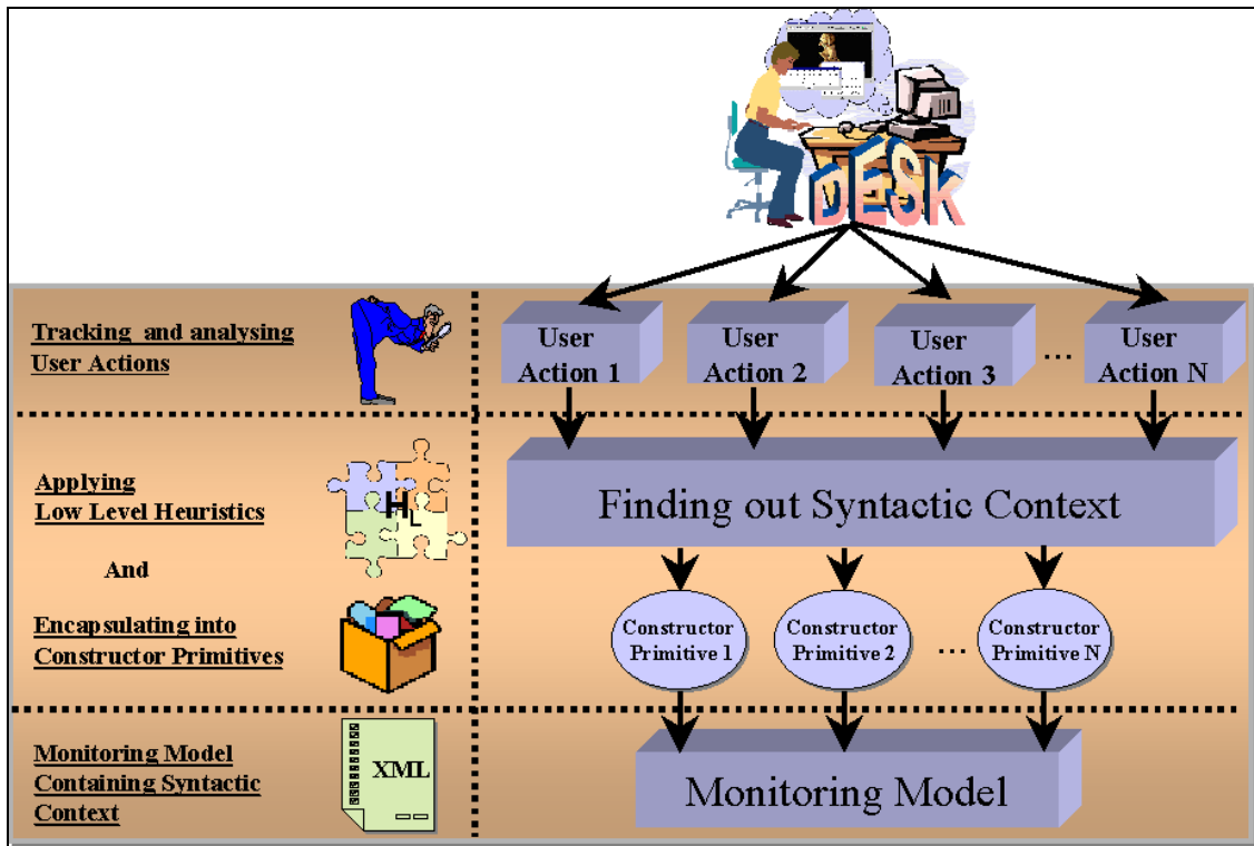
Figure 4. DESK client-side
