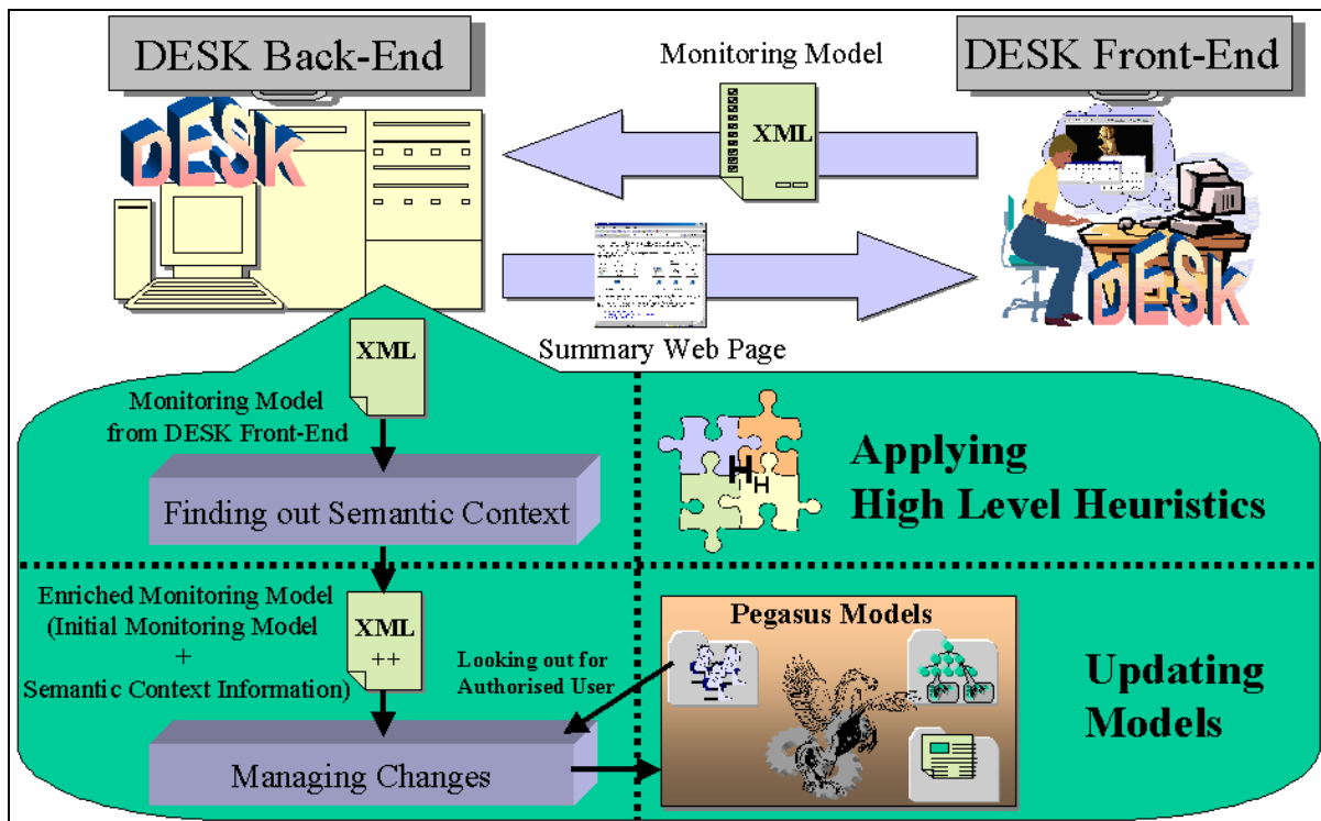
Figure 5. DESK server-side
