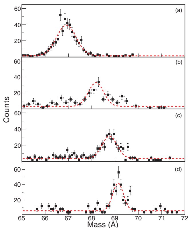
FIG. 2. (Color online) Mass spectra in coincidence with the observed delayed \gamma rays. The coincidence gates select (a) the 313 + 694-keV transitions in ^{67}\text{Ni} , (b) the 168-keV transition, (c) the ^{69}\text{Cu} lines, and (d) the 143 + 593-keV transitions in ^{69}\text{Ni} .
