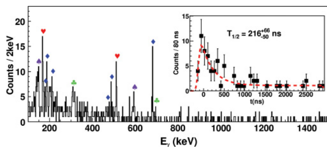
FIG. 1. (Color online) Delayed \gamma -ray spectrum in coincidence with ^{68}\text{Ni} . The purple spades, the blue diamonds, and the green clovers indicate, respectively, the ^{69}\text{Ni} , ^{69}\text{Cu} , and ^{67}\text{Ni} isomeric decay. The red hearts overscore the transition that belongs to ^{68}\text{Ni} . The inset shows the time spectrum from which the half-life of the 168(1)-keV transition is extracted.
