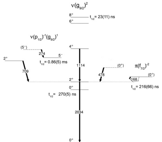
FIG. 3. Proposed level scheme deduced from the present work in ^{68}\text{Ni} . The open (solid) arrows indicate, respectively, the observed (prompt) \gamma ray. The configurations which are discussed in the text and isomer half-lives are indicated.
