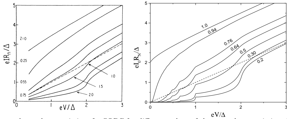
FIG. 2. dc current-voltage characteristics of a SQPC for different values of the normal transmission. Left panel corresponds to the semiclassical OTBK theory and right panel to the fully quantum mechanical calculation.
