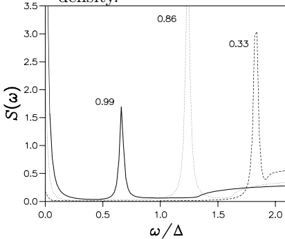
FIG. 6. Power spectrum S(\omega) of the zero-voltage current-fluctuations at k_B T = 0.2\Delta in a SQPC for three transmission values. The contact is biased at the maximum supercurrent.
