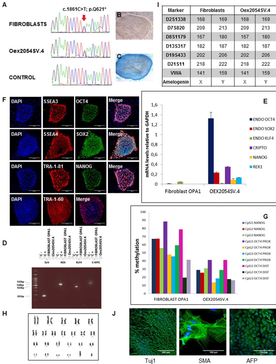
Fig. 1. Molecular and functional characterization of the Oex2054SV.4 iPSC line. A. Electropherograms showing the mutation in the patient's fibroblasts and in the Oex2054SV.4 line. B. Typical ES-like colony morphology of the Oex2054SV.4 iPSC line. C. Positive phosphatase alkaline staining. D. RT-PCR for detecting the clearance of the vectors and the exogenous reprogramming factor genes. E. QPCR showing the expression of the pluripotency associated markers NANOG , OCT4 , SOX2 , KLF4 , CRIP1O and REX1 . F. Immunofluorescence analysis showing expression of typical pluripotent ES cell markers such as the transcription factors OCT4 , NANOG , SOX2 and the surface markers SSEA3 , SSEA4 , TRA1-60 and TRA1-81 ; scale bars: 300 \mu m. G. Bisulfite pyrosequencing of the OCT4 and NANOG promoters. The promoters of the transcription factors, OCT4 and NANOG , were almost demethylated in the generated iPSC line. H. Karyotype analysis. Oex2054SV.4 has a normal karyotype (46, XY). I. DNA fingerprinting analysis showing that Oex2054SV.4 comes from the patient's fibroblasts. J. Embryoid body based in vitro differentiation assays. Oex2054SV.4 differentiates into all three germ layers, demonstrated by positive AFP endoderm staining, positive Tuj1 ectoderm staining and positive SMA mesoderm staining.
