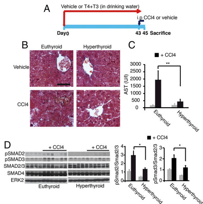
Fig. 7. Administration of thyroid hormones attenuates the acute hepatic response to CCl 4 treatment in mice. (A) Scheme of the treatments (vehicle, n = 4 ; CCl 4 , n = 6 ). (B) Representative Masson's trichrome staining of livers of the different experimental groups after acute CCl 4 treatment, showing extensive damage with nuclei loss only in euthyroid animals. (Scale bar, 50 \mu m.) (C) AST activity in serum. Data are mean \pm SEM. Significance of ANOVA posttest (Bonferroni) between euthyroid and hyperthyroid CCl 4 -treated mice is indicated. (D) Western blot of pSMAD2, pSMAD3, SMAD2/3, and SMAD4 in the livers after acute CCl 4 treatment. ERK2 was used as a loading control. (Right) pSMAD2/SMAD2,3 and pSMAD3/SMAD2,3 ratios (mean \pm SEM) were quantitated and are shown.
