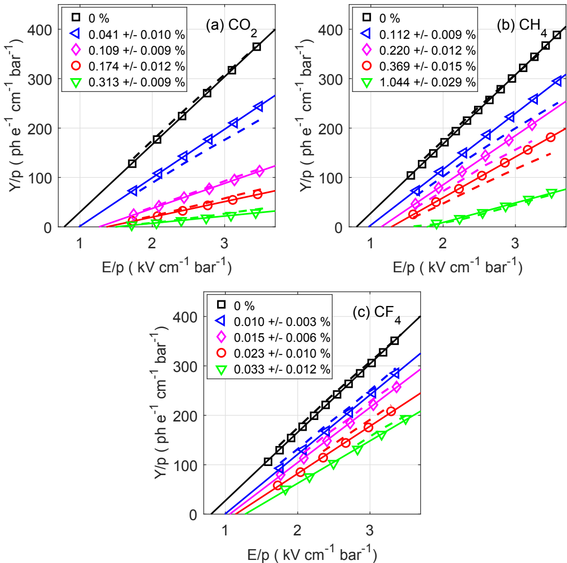
Figure 3: Reduced EL yield obtained for 5.9 keV x-rays, Y/p , as a function of the reduced electric field, E/p , for different concentrations of molecular gases added to pure xenon: (a) CO 2 ; (b) CH 4 ; (c) CF 4 . Total pressures of 1.13, 1.25 and 1.24 bar were used, in average, for Xe-CO 2 , Xe-CH 4 and Xe-CF 4 mixtures, respectively. Solid lines show linear fits to the data, while dashed lines are simulation values obtained with the code developed in [32].
