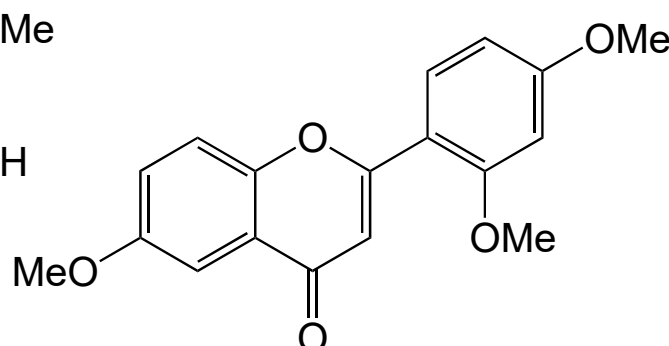
Trimethoxyflavone
