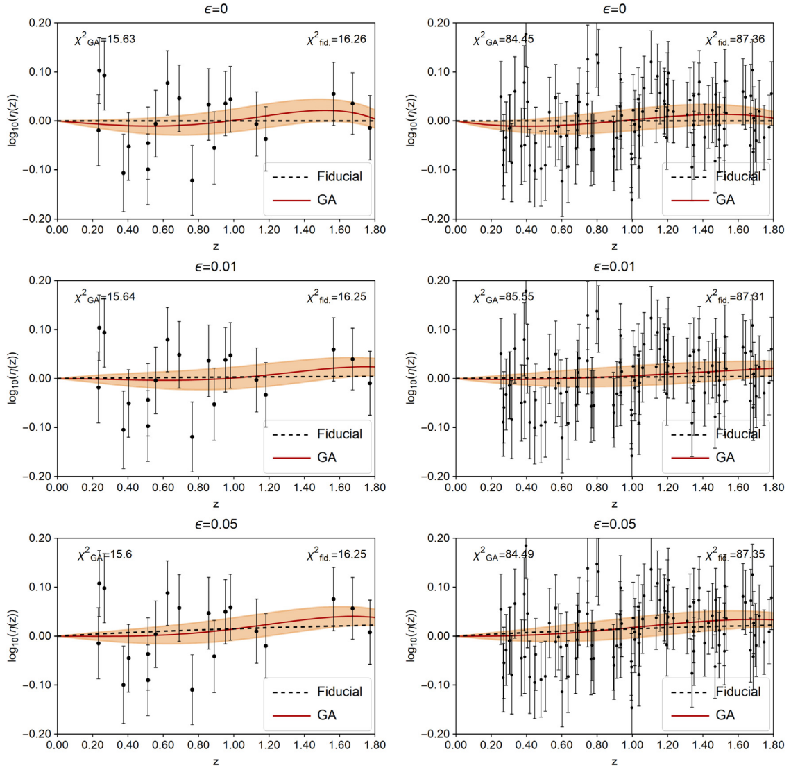
Fig. 2. The GA reconstructions for the 20 lenses (left column) and for 100 lenses (right column). The mocks in the top row were created with \epsilon = 0 , the ones in the middle row with \epsilon = 0.01 , while the ones in the bottom row with \epsilon = 0.05 . The orange shaded regions show the 1\sigma error for the GA, while the dashed black lines show the fiducial model, \log_{10}(1+z)^{\epsilon_0} , in each case.
