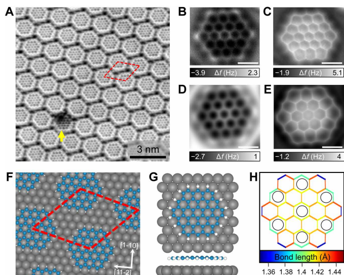
Fig. 2. Bond-resolved ncAFM imaging of the circumcoronene superlattice. (A) Large-scale ncAFM image of the circumcoronene array, collected with a CO-decorated tip. Defective circumcoronene molecule (indicated by yellow arrow) constitutes an approximately 2% of total products. (B and C) Constant-height ncAFM images of individual circumcoronene molecule, collected at tip-sample distances z = 40 pm in (B) and z = 60 pm in (C) with respect to set point V = 20 mV; I = 1 nA. (D and E) ncAFM images simulated using a numerical probe-particle approach, for a physical tip-sample distance of 0 pm in (E) and 20 pm in (D) with respect to set point 14.4 Å. (F) DFT-relaxed model of the circumcoronene-based superlattice on Cu(111). (G) Top view and side view of the single circumcoronene molecule on Cu(111). (H) DFT (B3LYP) calculations of the bond lengths within the circumcoronene molecule. Scale bars (B to E), 500 pm.
