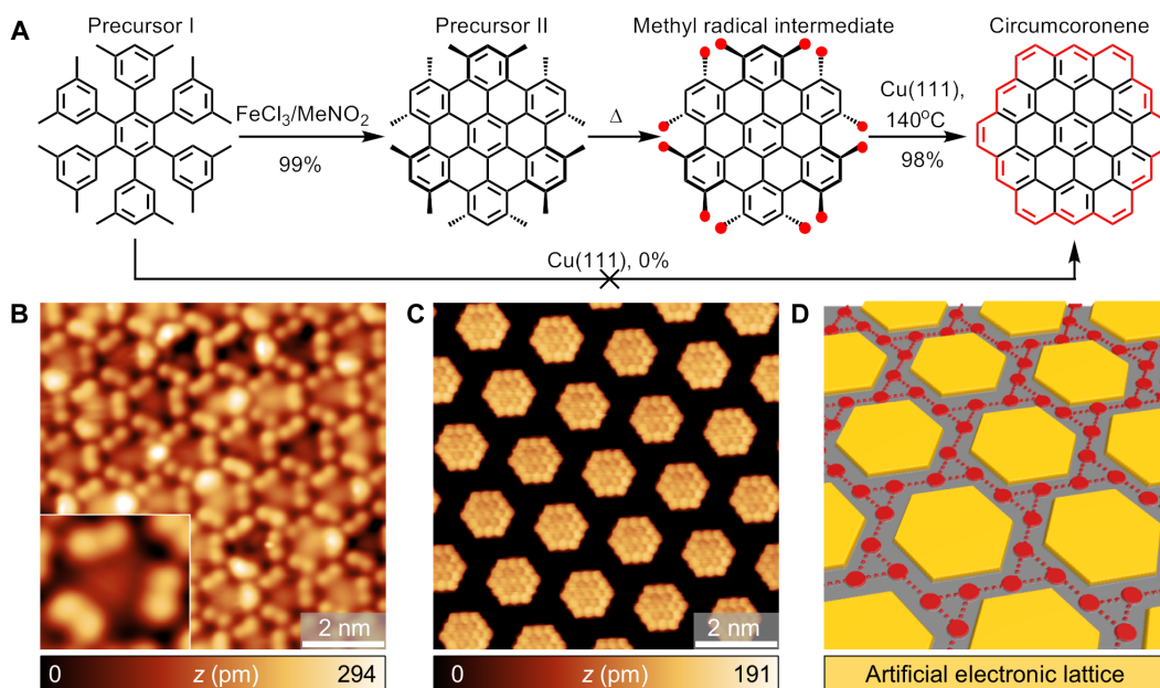
Fig. 1. On-surface synthesis of circumcoronene-based superlattice. (A) Precursor molecule II undergoes cyclodehydrogenation on Cu(111) via methyl radical-radical coupling toward formation of the circumcoronene. The cyclodehydrogenation results in ultrahigh-yield circumcoronene molecules. (B) STM image acquired after deposition of the precursor II onto Cu(111) at room temperature. Inset shows the STM image of an individual precursor molecule. (C) STM image collected after sample annealing at 140°C, revealing the presence of the circumcoronene-based self-assembly on Cu(111). (D) Schematic illustration of the chiral Kagome-honeycomb lattice.
