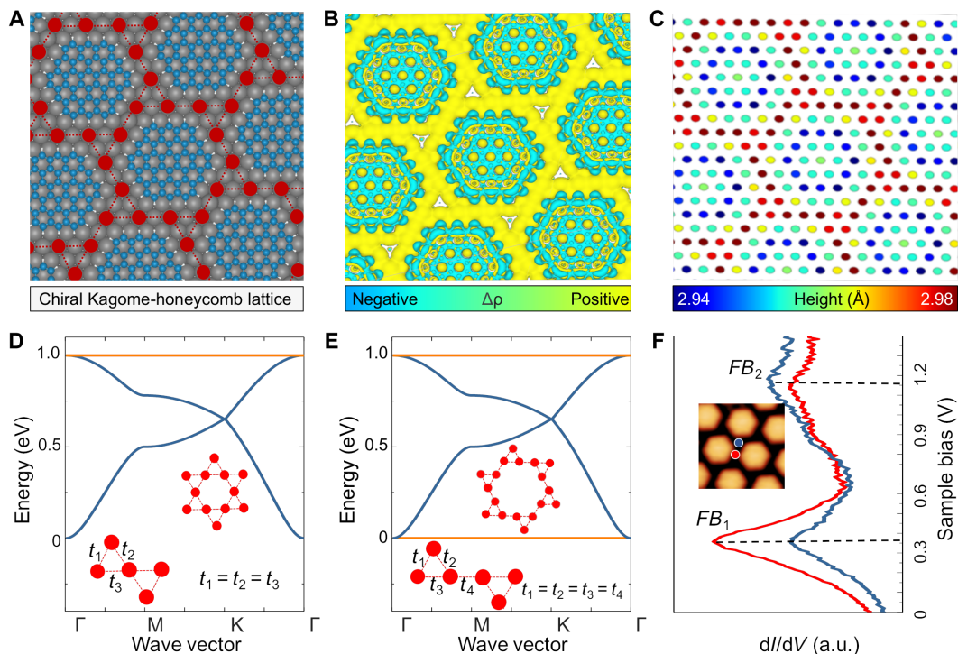
Fig. 4. Origin and electronic structure of the chiral Kagome-honeycomb lattice. (A) Schematic illustration of the chiral Kagome-honeycomb lattice. (B) Electrostatic potential of the circumcoronene superlattice. (C) The out-of-plane buckling of Cu atoms in the topmost Cu(111) layer. (D and E) A k -space dispersion of the electronic bands of the Kagome and chiral Kagome-honeycomb lattices, calculated using the TB model for hopping constants t_1 = t_2 = t_3 = -0.5 eV (D) and t_1 = t_2 = t_3 = t_4 = -0.5 eV (E). (F) Experimental dI/dV spectra reveal the existence of two characteristic peaks ( FB_1 and FB_2 ) associated with two flat bands of the chiral electronic Kagome-honeycomb lattice.
