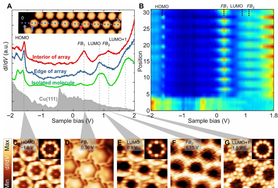
Fig. 3. Electronic structure of the circumcoronene array. (A) dI/dV spectra collected over the bare Cu(111) substrate (gray), a circumcoronene molecule residing at the periphery of the superlattice (blue), a circumcoronene molecule located in the interior of the superlattice (red), and an isolated molecule (green). a.u., arbitrary units. (B) 2D contour plot of dI/dV spectra acquired along the line indicated in the inset in (A). (C to G) Topography STM image (1 V; 1 nA) and corresponding dI/dV maps collected at energetic positions of states HOMO (C), FB_1 (D), LUMO (E), FB_2 (F), and LUMO+1 (G). Inset images in (C), (E), and (G) are the calculated dI/dV maps of the HOMO (C), LUMO (E), and LUMO+1 (G) of the circumcoronene using a CO-decorated tip.
