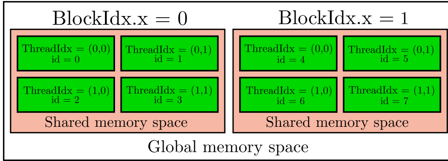
Figure 1.3: Representation of the thread geometry for a kernel launch with 2 blocks of 4 threads ( blockDim = (2,2) ). Threads inside the same block run concurrently, while different blocks might run desynchronized between them. Each thread has a small local (and private) register memory space. Furthermore, threads inside the same block can share memory among them via the low-latency shared memory . All threads can access the same, low-bandwidth, global memory space.
