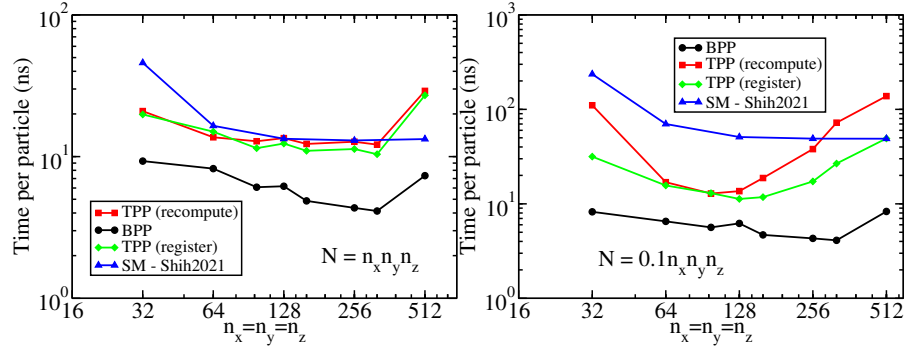
Figure 21.4: The same situation as in Fig. 21.3, but in this case particles are presorted to increase spatial locality in memory (particles close in space are placed close in memory). Both the positions and the spread quantity are sorted. Sorting is carried out using the same Morton hash technique laid out in chapter 11.2. Sorting takes a negligible amount of time and, moreover, it does not need to be done every time spreading occurs. Typically particles are sorted at the start of a given simulation and then every few diffusive times.
