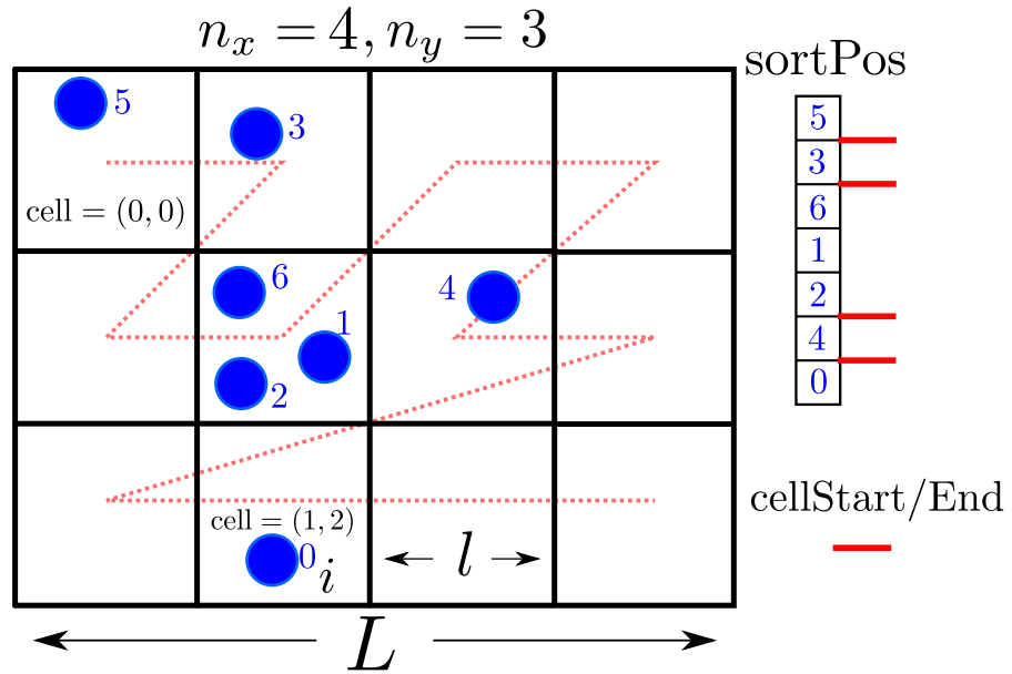
Figure 11.3: Representation of the spatial binning for a 2D distribution of particles. The particle marked as i lies in the cell with coordinates (1, 2) , these coordinates will then be used to assign a hash to particle i . The dotted red line represents the order given by the space-filling curve, starting at the (0, 0) cell. Blue particles lie in arbitrary indexes, aka memory locations, (blue numbers). After hashing the positions according to the red dashed line and sorting, particle positions of particles in the same cell are stored contiguously in sortPos (right), particles inside the same cell have an undetermined order. Solid red lines mark the end of a cell or, equivalently, the start of the next one, information that is stored in the cellStart and cellEnd arrays.
