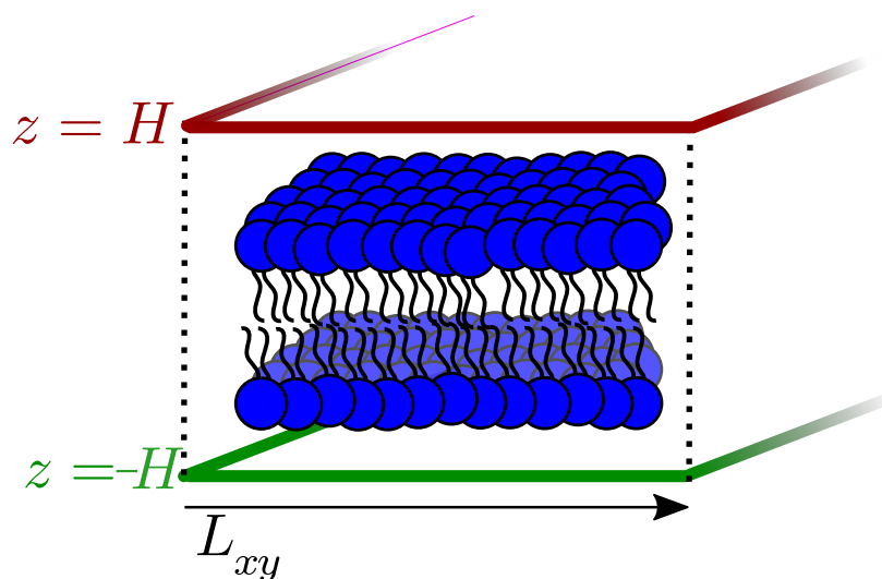
Figure 23.1: Representation of a lipid membrane inside a doubly periodic domain. The Boundary Conditions (BCs) can be customized at the domain limits ( z = -H, H ) to be either open or have no-slip walls.
