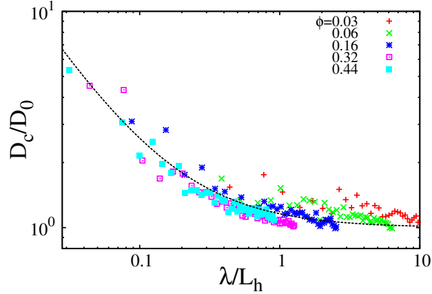
Figure 28.1: Collective diffusion, D_c(k) , of a group of ideal colloids under strict confinement ( \delta \rightarrow 0 ) for several densities. Dashed line correspond to D_c/D_0 = 1 + \frac{\lambda}{2\pi L_h} . Here L_h := \frac{2a}{3\phi} is the hydrodynamic length and \lambda := \frac{2\pi}{k} is the wavelength of a density perturbation. Note that for \lambda \rightarrow \infty , D_c \rightarrow D_0 , corresponding to the single particle diffusion coefficient, i.e. in this limit there are no collective effects (in the case of ideal particles).
