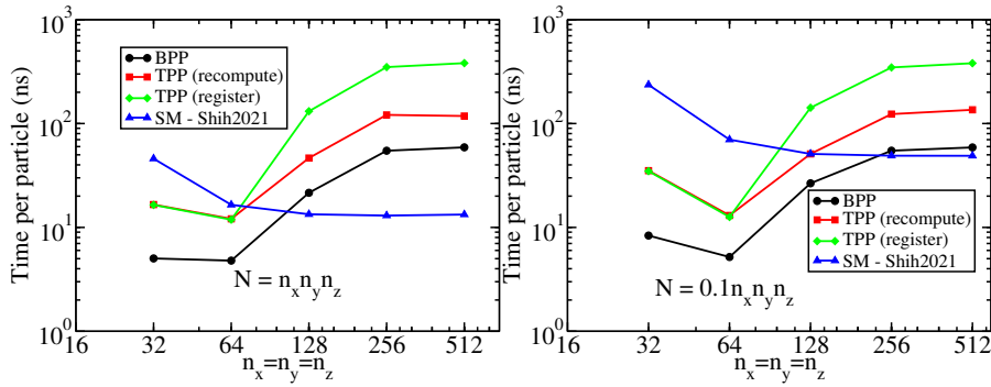
Figure 21.3: Performance comparison between the different spreading schemes considered for two different densities. Particles are distributed uniformly on a cubic grid and spread with a support n_s = 8 using a Gaussian kernel. A single scalar is spread per particle. The considered algorithms are: A block-per-particle (BPP), the algorithm used in UAMMD . A thread-per-particle (TPP) precomputing the kernel to register memory (register, similar to GM-sort in Shih2021 [118] ) and recomputing it (recompute). Finally, timing for the BDP algorithm ( SM in [118] ) is also presented. For these tests, particle sorting was not employed, i.e. the particles are randomly distributed in memory with respect to their physical positions. Performance data was gathered in an RTX2080Ti GPU using single precision. The crossover between BPP and SM happens at around 2 million particles in both cases.
