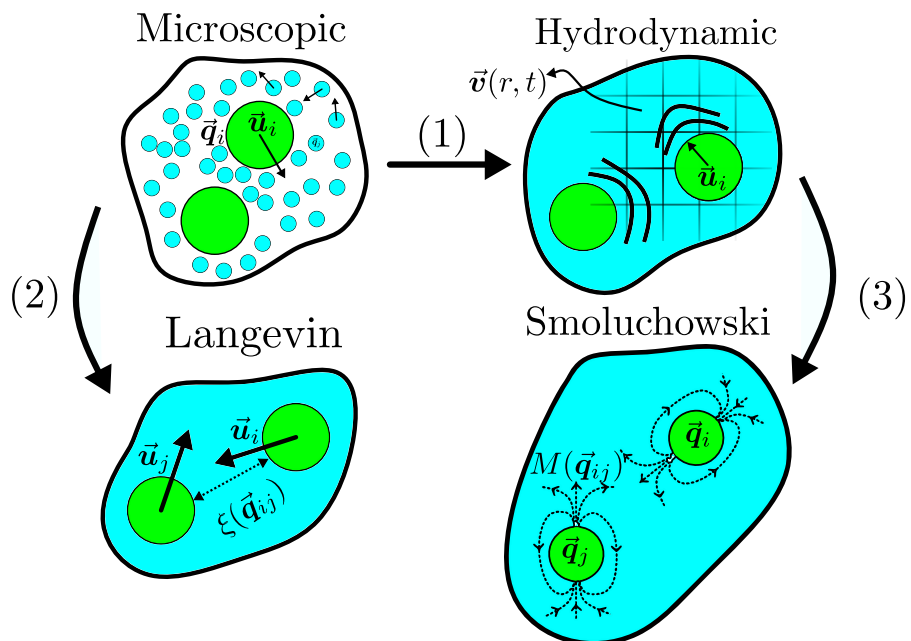
Figure 3.3: The different levels of coarse grained description available in UAMMD for soft matter simulations. \mathbf{q}_i represents the positions of particles, \mathbf{u}_i their velocity. \mathbf{v}(\mathbf{r}, t) represents an Eulerian fluid velocity field, M(\mathbf{q}_{ij}) a mobility tensor and \xi(\mathbf{q}_{ij}) a friction kernel. Arrows represent standard routes for the formal bottom-up derivation using coarse-graining theory. In order, we have: (1) in [25], (2) in [26] and (3) in [27].
