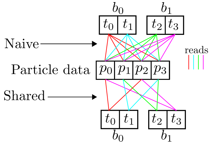
Figure 9.2: Representation of algorithms 2 (upper half of the figure) and 3 (bottom half). Two thread blocks ( b_{0,1} ), with two threads each ( t_{0,1,2,3} ), have to process four particles ( p_{0,1,2,3} ). Each thread must go through all particles and fetch some arbitrary information for each of them (i.e. positions, velocities and/or any other data required by the computation), represented by colored lines. The naive algorithm does not make use of the shared memory space available to threads in the same block and thus each thread needs to read all particles. On the other hand, the shared algorithm benefits from the shared memory space. In particular, each particle must be fetched only once per block (as opposed to once per thread in the naive algorithm). This is depicted by the reduced number of colored lines in the lower side of the figure.
