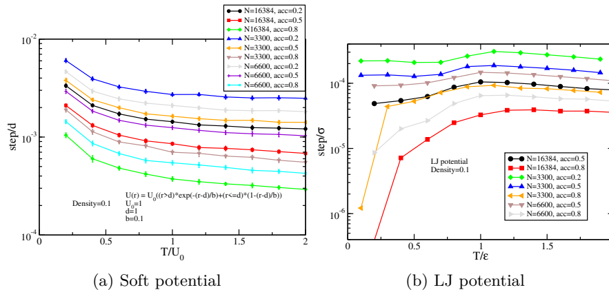
Figure 17.1: Optimal time step in MALA for several acceptance ratios and number of particles using a soft repulsive potential (left) and a hard steric WCA interaction (right). Naturally, a higher acceptance ratio (with corresponding 1 to accepting all configurations and 0 to never accepting them) results in a lower \delta t . A by-product of the MALA algorithm comparing the total energy change is that \delta t depends on the number of particles so that more particles result in a lower optimal \delta t .
