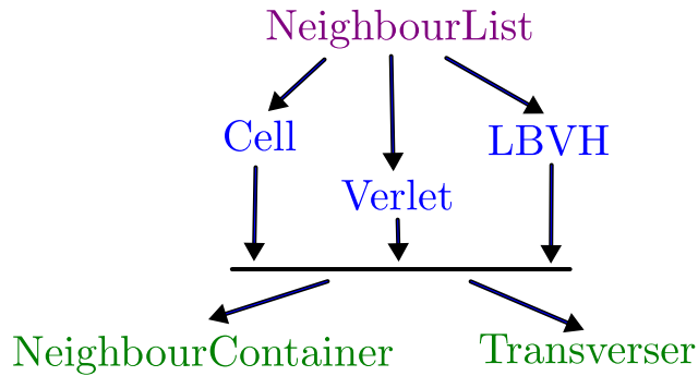
Figure 11.2: The three types of neighbour lists in UAMMD. All of them can be used via the same unifying interfaces; Transverser (described in Appendix E.1) and NeighbourContainer (described in sec 11.1). Additionally, the internal structures of each list can be requested for custom use.
