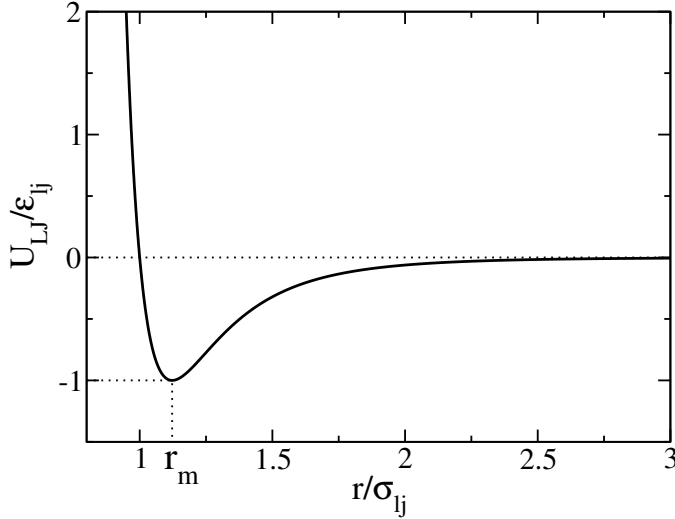
Figure 10.1: The Lennard-Jones potential described in Eq. 10.1
