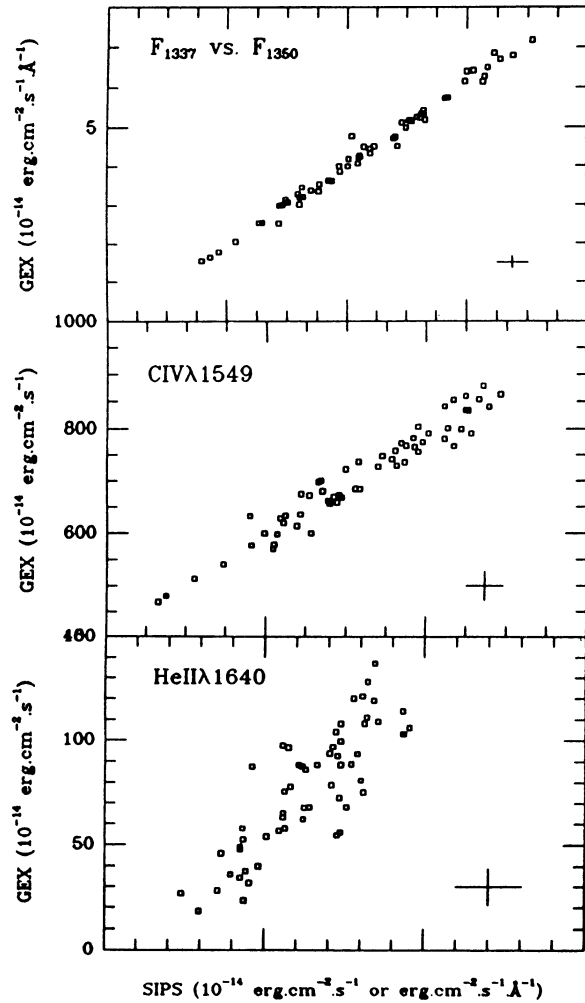
FIG. 2.—Flux, as obtained with GEX, plotted as a function of the SIPS flux for the continuum near 1300 Å (upper panel), the C IV 1549 emission line (middle panel), and the He II 1640 + O III] 1663 blend (lower panel). A typical error bar is shown in the lower right-hand corner of each panel. The scale is such that the range covered is the same along the X- and the Y-axis.
