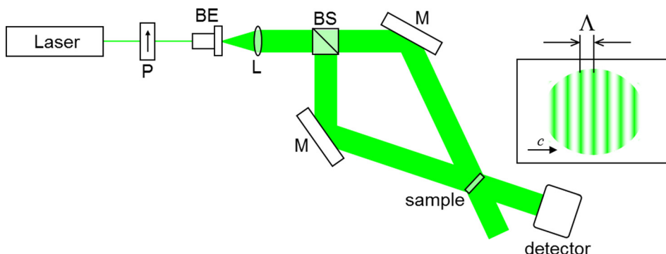
FIG. 6. Experimental setup for holographic illumination. P polarizer, BE beam expander, L lens, BS beam splitter, and M mirrors. Reprinted with permission from Burgos et al. , Opt. Mater. 35, 1700 (2013). Copyright 2013 Elsevier.
