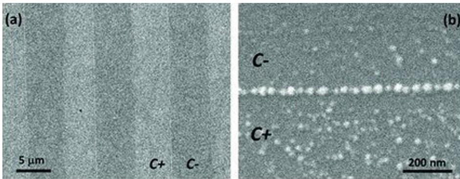
FIG. 18. (a) SEM image of the surface of a \text{Nd}^{3+} doped PPLN crystal after selective photochemical deposition of Ag NPs; dark regions correspond to c^- domain surfaces with a low Ag NP density; light regions are c^+ domain surfaces with a higher density of Ag. (b) Higher resolution SEM image showing a domain boundary on which a chain of Ag nanoparticles has been formed. Reprinted with permission from Yraola et al. , Adv. Mater. 25 , 910 (2013). Copyright 2013 John Wiley and Sons.
