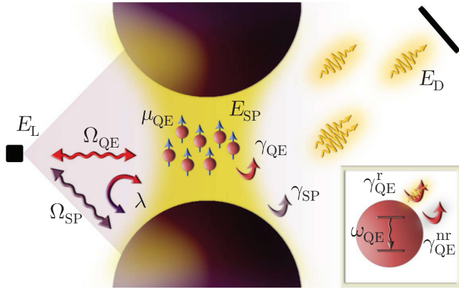
Fig. 1. A QE ensemble resonantly coupled to a generic plasmonic cavity. The right inset depicts the two-level QE model.
