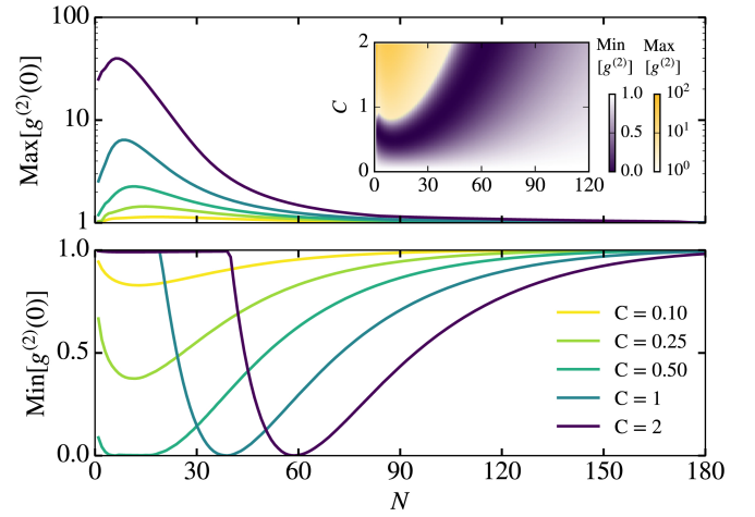
Fig. 4. Maximum (top) and minimum (bottom) correlation function as a function of the QE ensemble size for several values of the single emitter cooperativity. The inset in the upper panel shows the map of photon positive (yellow) and negative (violet) correlations as a function of N and C .
