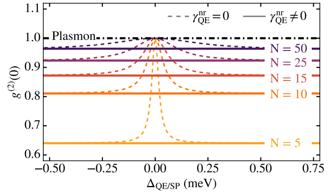
Fig. 2. Correlation function g^{(2)}(0) versus laser detuning for SP (black dash-dotted line) and QEs (color lines) uncoupled. Various ensemble sizes are shown, with (solid) and without (dashed) the inclusion of QE nonradiative decay, \gamma_{\text{QE}}^{\text{nr}} .
