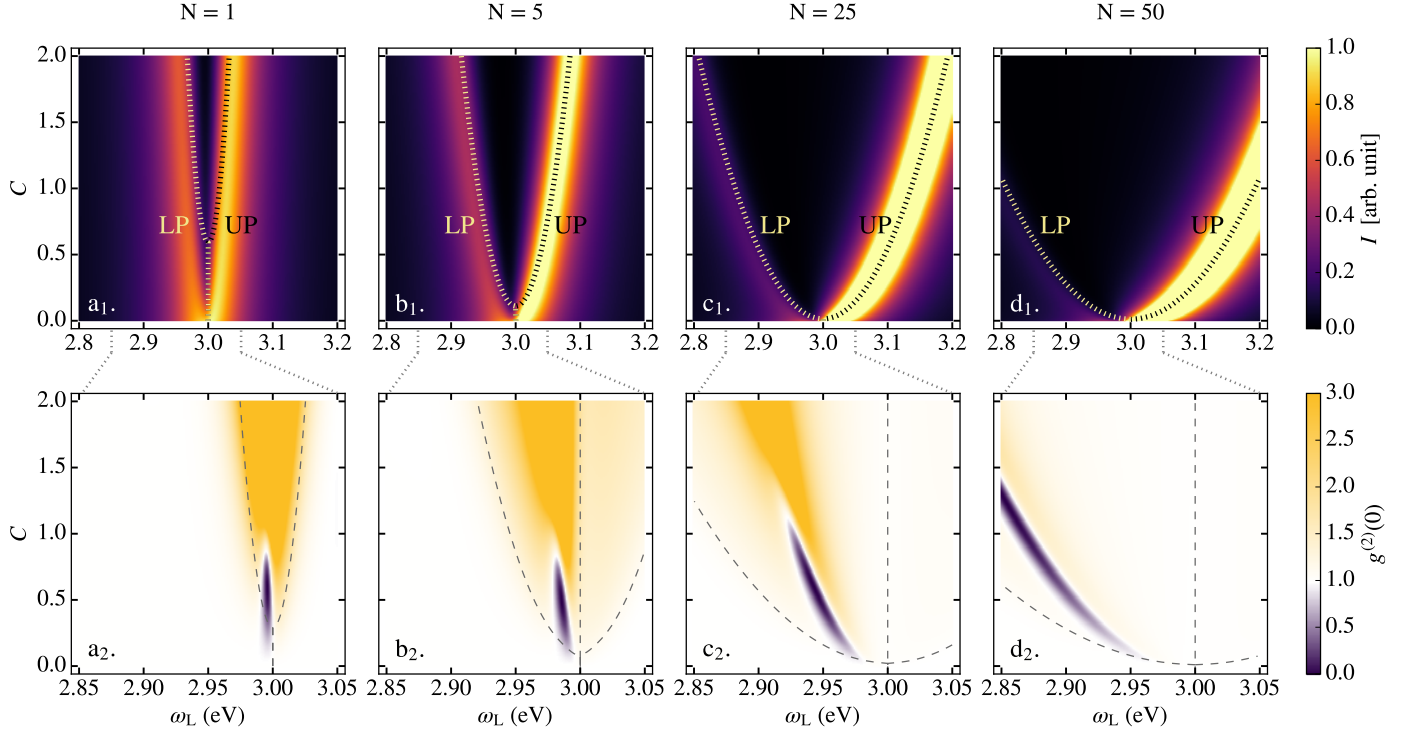
Fig. 3. Scattering intensity I (a 1 -d 1 ) and correlation function g^{(2)}(0) (a 2 -d 2 ) versus laser frequency and single emitter cooperativity for various QE-SP systems. In the upper (lower) panels dotted (dashed) lines plot the PEP frequencies (half frequencies) in the one-excitation (two-excitation) manifold.
