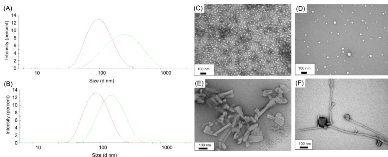
Figure 4. (A, B) DLS results for compounds (A) 1A and (B) 1T , at low (i.e., 120 \mu\text{M} for 1A and 10 \mu\text{M} for 1T – green curves) and high concentration (500 \mu\text{M} – red curves). (C-F) Representative TEM micrographs of the spherical, rectangular and fibrillar assemblies formed by (C) 1A , (D) 1A* (E) 1T , and (F) the mixture 1A-1T , respectively. For the 1A-1T mixture, it was not possible to obtain DLS data with good correlograms, due their fibrillar nature, yet signals corresponding to much larger and polydisperse structures were identified.
