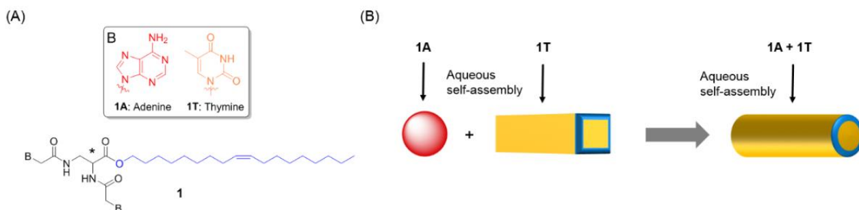
Figure 1. (A) Structure of dinucleolipids 1A and 1T , presenting complementary nucleobases in each of their respective polar heads: two adenine (for 1A ) or two thymine (for 1T ) moieties, respectively. (B) Cartoon showing the strategy to study the types of nanostructures yielded by 1A (spherical assemblies) and 1T (crystal-like rectangular assemblies) in aqueous medium, and their transformation into a third type of structure (fibrillar assemblies) when they are mixed.
