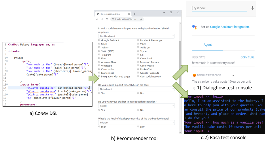
Fig. 5: Our tool in action for forward engineering. (a) CONGA editor. (b) Recommender. (c.1) Generated bot for Dialogflow. (c.2) Generated bot for Rasa.
