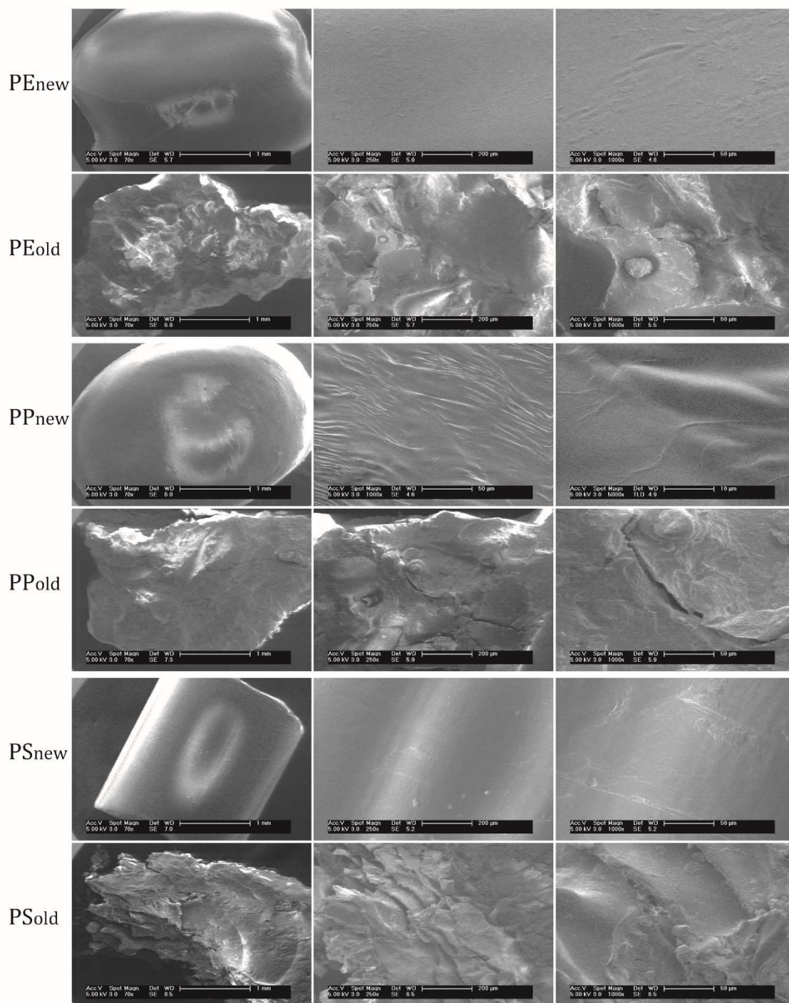
Figure S7. SEM images of sampled plastic particles (aged) compared with pristine (new) pellets of the same composition.
