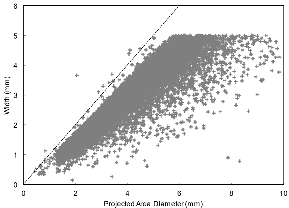
Figure S5. Comparison between particle width (directly from particle images) with projected area diameter calculated as the diameter of the circle with the same area as the particle.
