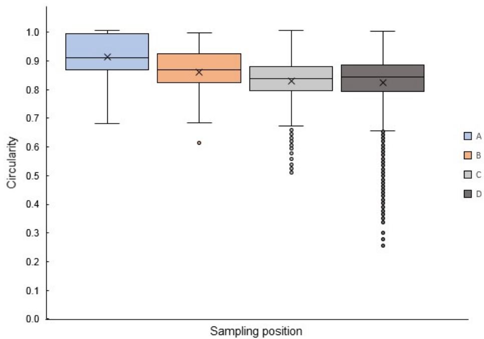
Figure S6. Circularity for plastic particles sampled indicating average, median and outliers.
