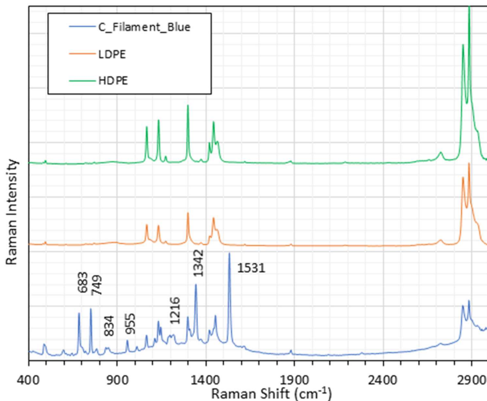
Figure S8. Comparison images between Raman spectra (785 nm) from a blue filament and PE spectra. Spectra changes have been identified as belonging to cooper phthalocyanine (88 % similarity from Lens Raman library database).
