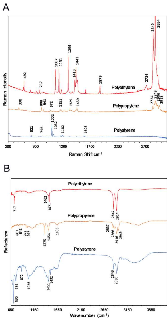
Figure 4. Raman (A) and ATR-FTIR (B) representative spectra of different sampled microplastic fragments identified as PE, PP and PS. because of its sensitivity to additives sometimes complicated the assessment of polymer characteristic bands. One example is shown in Fig. S8 (SM) in which cooper phthalocyanine, a blue colorant typically used in plastics, was identified (Caggiani et al., 2016; Ribeiro-Claro et al., 2017). The presence of additives is a subject topic of controversy as their leaking is a well-known cause for environmental concern (Koelmans et al., 2016; Whitmire et al., 2017).
