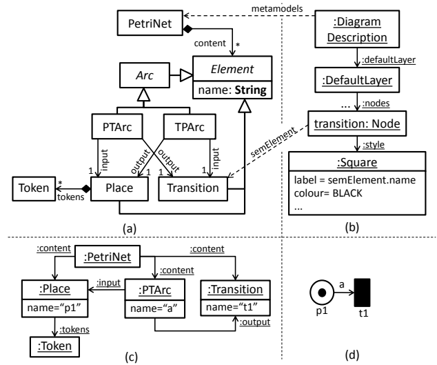
Figure 1. (a) Petri nets meta-model. (b) Excerpt of graphical concrete syntax definition. (c) Petri net model in abstract syntax. (d) Petri net model in concrete syntax.
