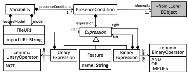
Figure 5. Variability meta-model.
