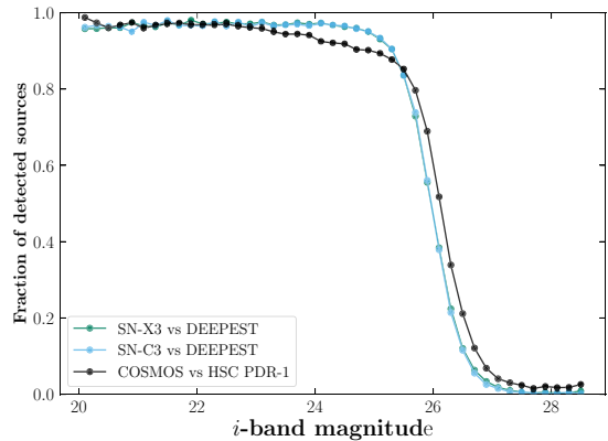
Figure 14. Detection completeness of sources in our Deep-Fields catalogue (COADD_TRUTH depth level) versus the DEEPEST level of coadd images (SN-X3, SN-C3) or HSC-PDR1 (COSMOS) as a function of magnitude. Deep-Fields masks were applied to the source lists, but some artefacts and spurious sources will remain in the DEEPEST and HSC data. The DEEPEST image in SN-E2 is not deep enough to produce a meaningful test for the COADD_TRUTH data. The data for SN-X3 and SN-C3 lie almost exactly on top of one another.
