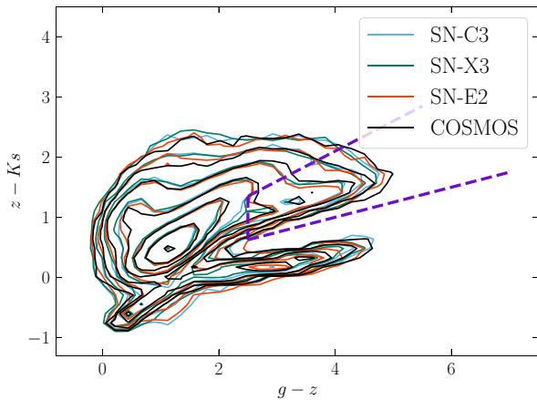
Figure 10. Selection diagram for the red-sequence galaxy population used in fine-tuning the interfield calibration. Similar to a BzK diagram (Daddi et al. 2004), the g-z and z-K colours cleanly separate the stellar locus from the galaxy population and allow the isolation of the red sequence at intermediate redshifts (Lane et al. 2007), shown by the purple dashed selection region. Galaxies in this sequence should have the same colours in different fields, and are used as part of our regression analysis.
