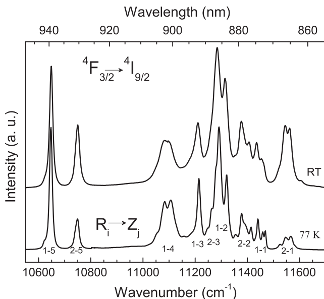
FIG. 2. Ambient pressure emission spectra of the ^4\text{F}_{3/2} \rightarrow ^4\text{I}_{9/2} transition at RT and 77 K. The identification of the \text{R}_{1,2} \rightarrow \text{Z}_{1-5} transitions is also given.
