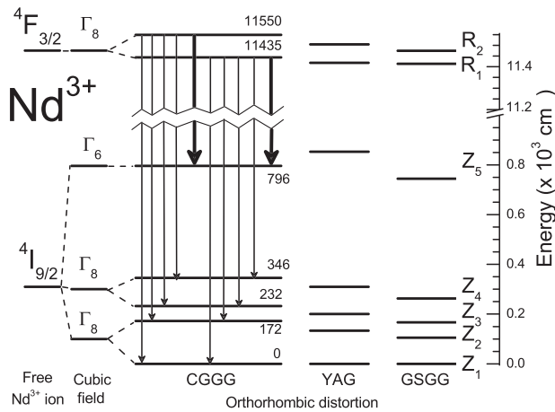
FIG. 1. Partial energy level diagram of the \text{Nd}^{3+} ion in CGGG, GSGG, 9 and YAG 10 garnets at ambient pressure corresponding to the ^4\text{F}_{3/2} and ^4\text{I}_{9/2} free- \text{Nd}^{3+} multiplets and the breakdown of their degeneracy into three and five Stark levels in cubic and orthorhombic-distorted environments, respectively. Due to the multi-site nature of the CGGG garnet, the energy of each \text{Nd}^{3+} Stark level indicated in the figure is averaged. The transitions between the ^4\text{F}_{3/2} and ^4\text{I}_{9/2} Stark levels are also given.
