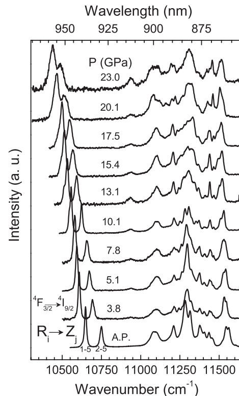
FIG. 3. Room temperature emission spectra of the ^4\text{F}_{3/2} \rightarrow ^4\text{I}_{9/2} transition as a function of pressure.
