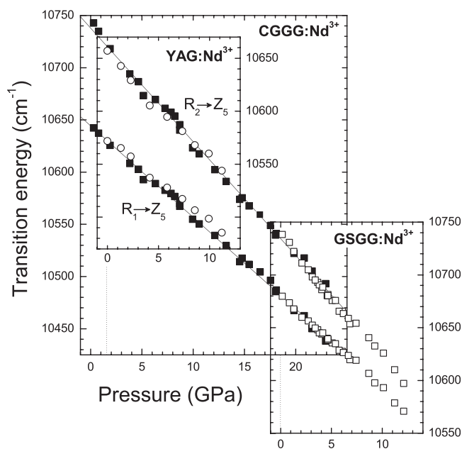
FIG. 5. Pressure evolution of the R_1, R_2 \rightarrow Z_5 peaks in \text{Nd}^{3+} -doped CGGG (■), GSGG (□), 9 and YAG (○). 10 All graphs use the same scale for the XY axes, but those for YAG and GSGG garnets are shifted in order to fit the same splitting as that of the CGGG garnet under study. Linear fits of the peak transition energies for the CGGG garnet are also included.
