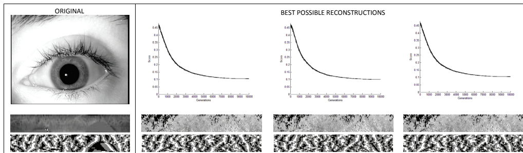
Figure 9: Three “best possible” reconstructions reached with the proposed algorithm (right) for the same original image (left). For the reconstruction samples, the evolution of the score through the generations is shown on top, with the final reconstructed normalized image and its corresponding iriscodes shown below.
