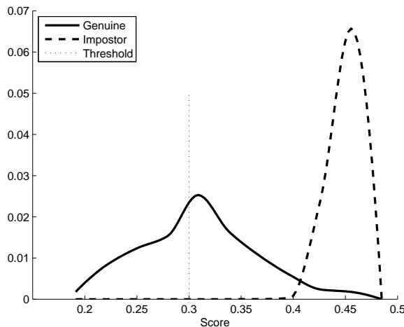
Figure 6: Genuine and impostor score distributions of the iris matcher used in the development experiments. The selected positive matching threshold is marked with a vertical dotted line, \delta = 0.3 .
