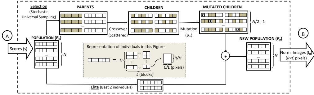
Figure 3: Diagram of the probabilistic method proposed in the present work for the reconstruction of iris images from their iriscode. Points A and B (input and output of the reconstruction algorithm respectively) may be seen for reference in Fig. 2. As is shown in the shaded chart in the center of the figure, although individuals are represented as vectors for simplicity, strictly they are matrices of size R \times C pixels divided into H \times L blocks.
