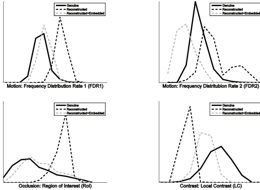
Figure 11: Distributions for the four quality features considered in the quality assessment study for the three databases used in the experiments.
