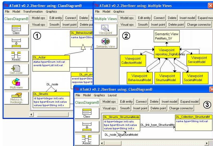
Fig. 6. Building the Environment for VisMODLE.
