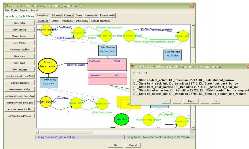
Fig. 15. Execution of Analysis Method Call.
