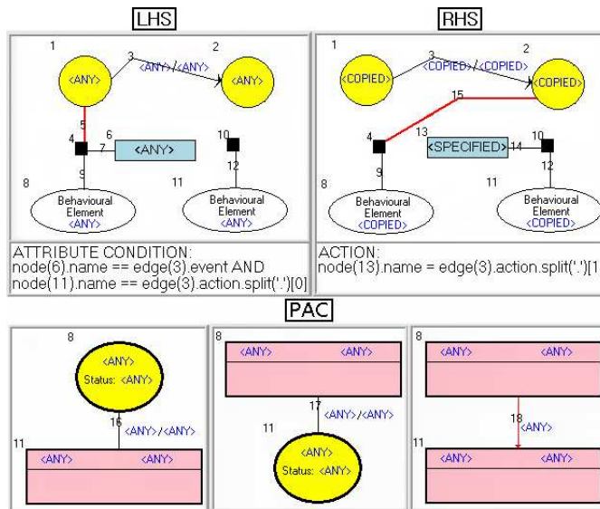
Fig. 11. Simulation Rule process event with action .
