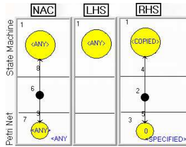
Fig. 12. Triple Rule SM state to PN place.
