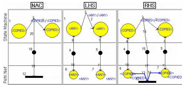
Fig. 13. Triple Rule SM transition to PN transition.
