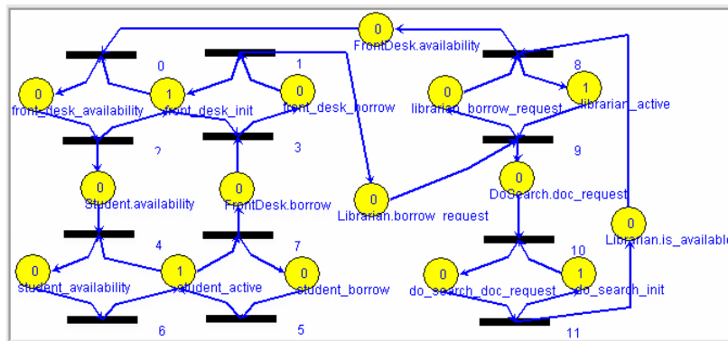
Fig. 14. Place/Transition Petri Net for the DL Example.
