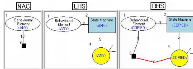
Fig. 9. Simulation Rule create input .
