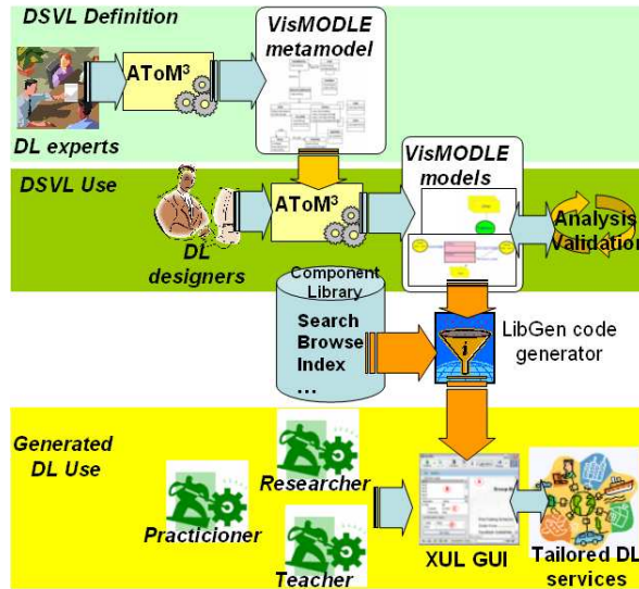
Fig. 5. The MDS Architecture for DLs.
