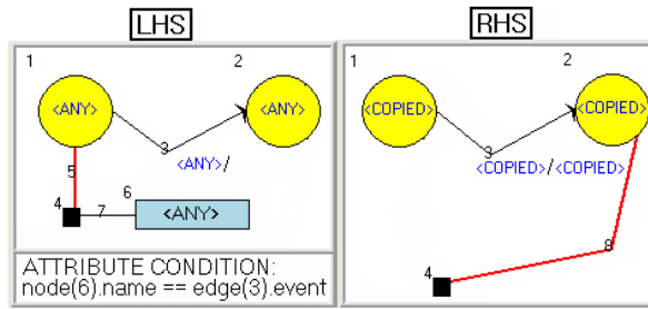
Fig. 10. Simulation Rule process event .
