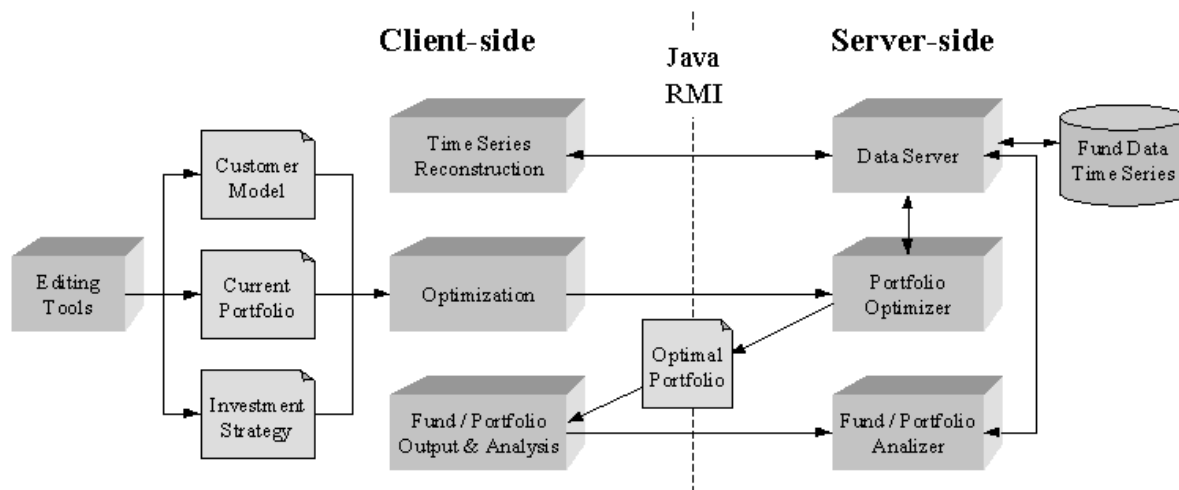
Figure 2 e-Portfolio Architecture
