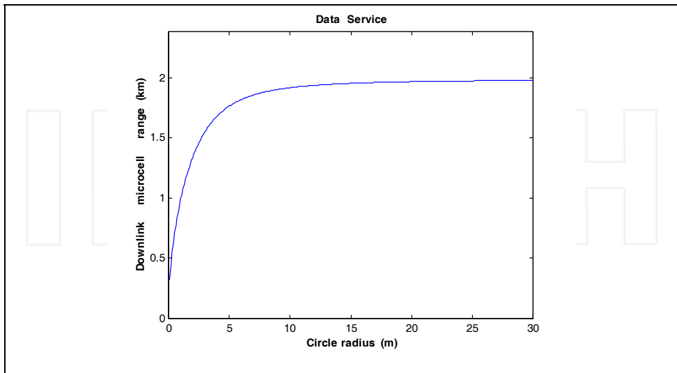
Fig. 8. Effect of the UWB interference on the UMTS microcell range as a function of the circle radius ( N = 6 , P_{\text{UWB}} = -55\text{dBm/MHz} ).
