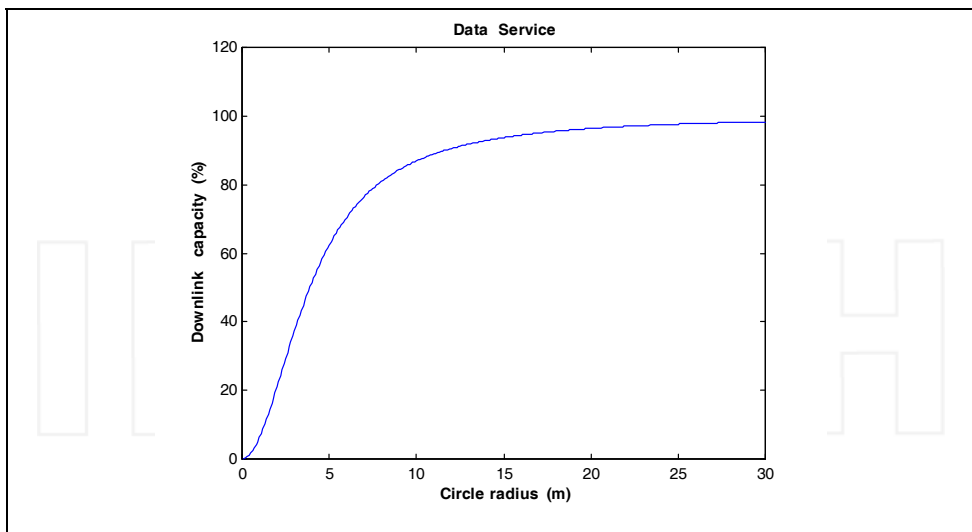
Fig. 9. Effect of the UWB interference on the UMTS microcell capacity as a function of the circle radius ( N = 6 , P_{\text{UWB}} = -55\text{ dBm/MHz} ).
