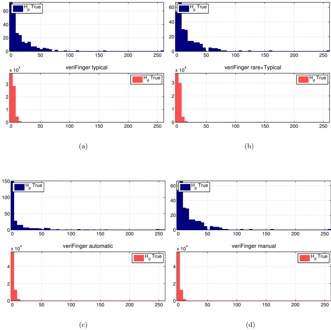
Figure 7.2: Histograms of pooled scores for (c) and VeriFinger-Typical (a), VeriFinger-Typical+Rare (b), VeriFinger-Automatic (c), VeriFinger-Manual (d).
