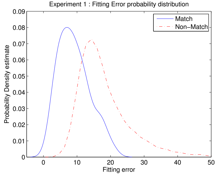
Figure 5.2: Probability density estimate of the fitting errors for match and non-match comparisons.
