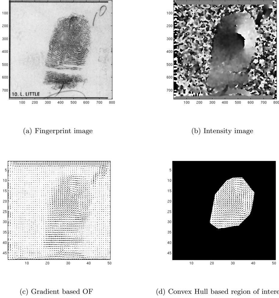
Figure 3.5: Gradient based orientation field estimated directly from fingerprint image. (a) is the gray scale fingerprint image. (b) and (c) shows the magnitude and angle of the orientation images obtained. (d) is the region of interest estimated from the convex hull of minutiae.
