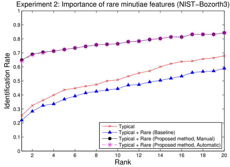
(a) CMC curve for NIST-Bozorth3
