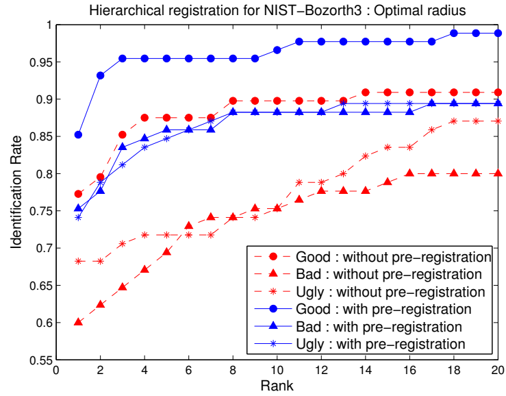
(a) NIST-Bozorth3 : Hierarchical registration with optimal parameters
