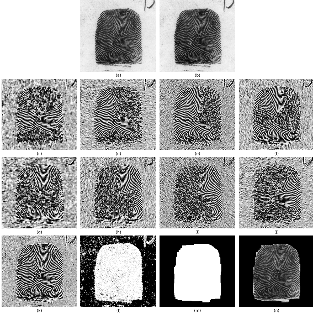
Figure 4.4: The various stages involved in generating the region of interest using gabor filter based segmentation. (a) original fingerprint image, (b) histogram normalized, (c)-(j) gabor responses for eight different orientations ( 0^\circ , 22.5^\circ , 45^\circ , 67.5^\circ , 90^\circ , 112.5^\circ , 135^\circ , 157.5^\circ ) respectively on normalized fingerprint image, (k) mean of all 8 different gabor responses, (l) gradient based thresholding, (m) ROI mask generated after performing erosion and dilation on (l), (n) the segmented fingerprint image.
