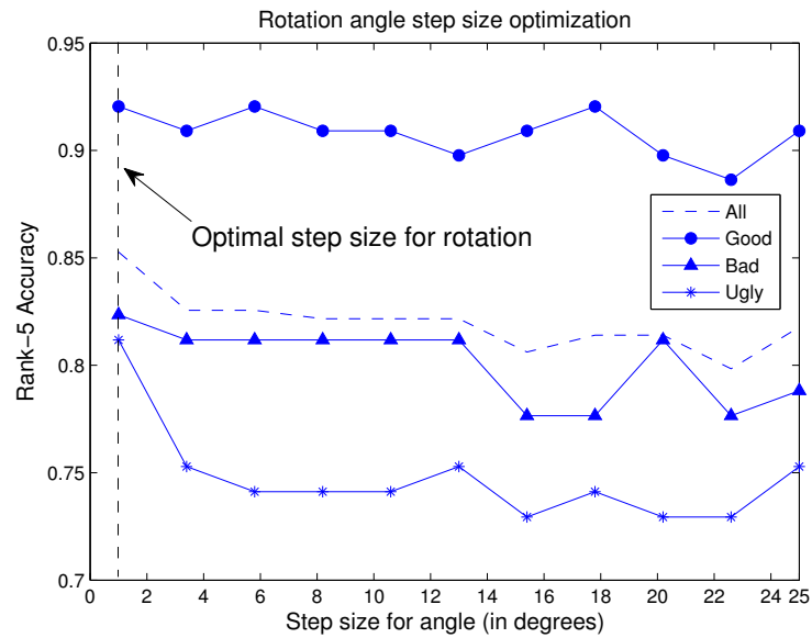
(a) Change in Rank-5 accuracies when increasing the step size in the range 1^\circ to 25^\circ
