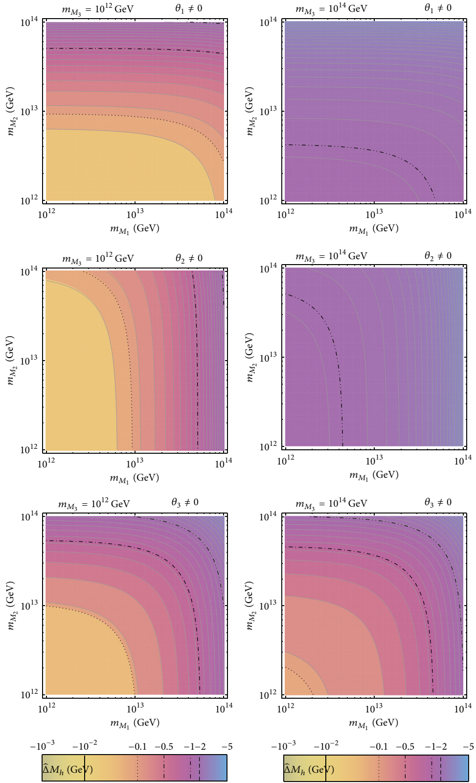
FIGURE 10: \widehat{\Delta}M_h contour lines in the (m_{M_1}, m_{M_2}) plane for two values of m_{M_3} and for a single complex nonvanishing \theta_i angle. Left panels: with m_{M_3} = 10^{12} GeV. Right panels: with m_{M_3} = 10^{14} GeV. Top panels: \theta_1 = 3\pi/4e^{i\pi/4} , \theta_2 = \theta_3 = 0 . Middle panels: \theta_2 = 3\pi/4e^{i\pi/4} , \theta_1 = \theta_3 = 0 . Bottom panels: \theta_3 = 3\pi/4e^{i\pi/4} , \theta_1 = \theta_2 = 0 . The rest of input parameters are set to the reference values in (79).
