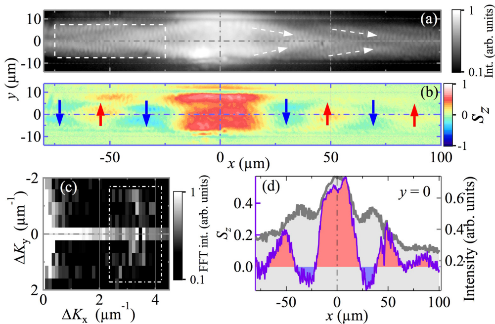
FIG. 4. (Color online) Collective polariton condensate spin precession in a quasi-1D ridge. (a) Polariton PL distribution in real space under nonresonant (1.612 eV), circularly polarized ( \sigma^+ ) excitation at the center of the ridge. The pump power is 3.75 \times P_{\text{th}} . Dashed white arrows sketch the direction of the polariton flow along its propagation. (b) Corresponding circular degree of polarization distribution ( s_z ). Vertical blue and red arrows highlight the spin precession, oscillating from negative ( \sigma^- ) to positive ( \sigma^+ ) values, respectively. (c) FFT intensity of the region enclosed by a dashed, white rectangle in panel (a). The dot-dashed, white rectangle marks the region of relevant frequencies arising from interferences between propagating and backscattered polaritons in real space. The PL and the FFT map are coded in a logarithmic, false color scale, while a linear one is used for s_z . (d) PL ( s_z ) vs x in the central region of the ridge y = 0 , plotted with a thick gray (thin purple) line.
