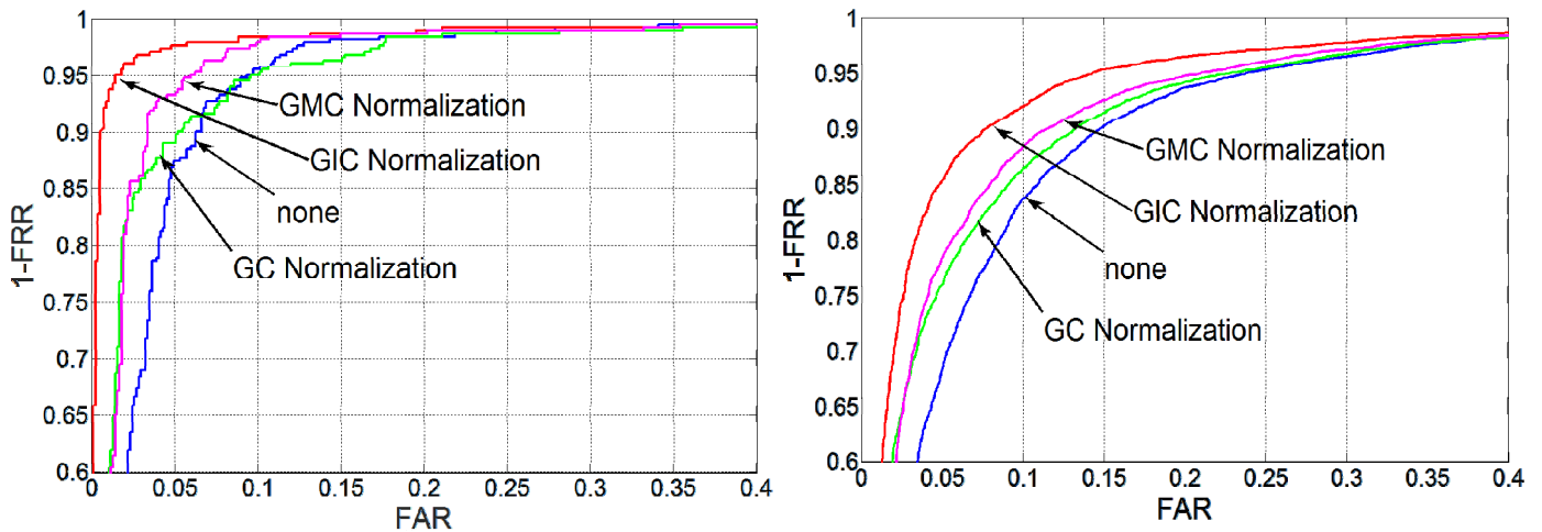
Figure 3: ROC curves for different normalization strategies using the Modified Scaled Manhattan Distance and ATVS-Keystroke database (on the left) and CMU database (on the right).
