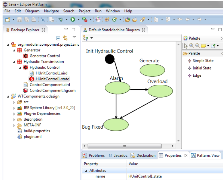
Fig. 6: Generated graphical modelling environment.
