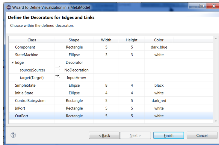
Fig. 5: Dedicated wizard for assigning a graph-based concrete syntax. Step 3: customization of appearance of nodes and edges.
