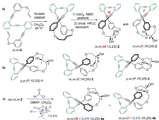
Fig. 1 Representative synthetic route (a) to enantiopure diol m,m -( M ,1 S ,2 S )-2 and m,m -( P ,1 R ,2 R )-2. (b) Structure of p,p -1, m,m -2 and p,m -3 enantiomers and (c) synthesis of diastereomeric (1' S ,4' R )-camphanoyl esters 4a and 4b.
