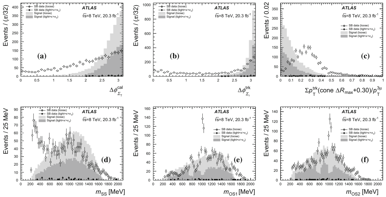
Fig. 4 The complementary variables used in the loose or tight selection but not as inputs for the BDT. \Delta\phi_{\Sigma_T}^{\text{cal}} in a , \Delta\phi_{\Sigma_T}^{\text{trk}} in b , \Sigma p_T^{\text{trk}} (\Delta R_{\text{max}}^{3\mu} + 0.30) / p_T^{3\mu} in c , m_{\text{SS}} in d , m_{\text{OS1}} in e and m_{\text{OS2}} in f . The loose data in the sidebands are shown as hollow circles , while the loose signal MC events are shown as light solid grey area . The tight+ x > x_0 data in the sidebands are shown as the solid black circles , while the tight+ x > x_0 signal
