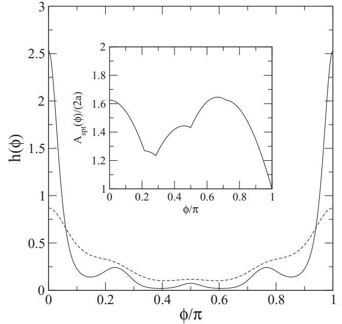
FIG. 9. Orientation distribution functions, h(\phi) for two coexisting nematics, N_1 (dashed) and N_2 (solid) of kites with \alpha_1 = 0.285\pi = 51.3^\circ and \alpha_1 + \alpha_2 = 180^\circ calculated from SPT. Inset: the SPT-area, A_{\text{spt}}(\phi) , for these kites.
